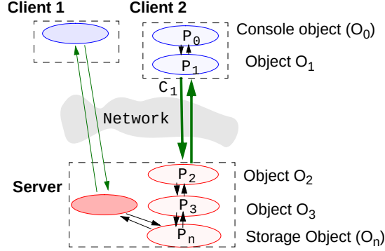
Figure 4: This figure shows how mobile objects interact in a layered system. Most of the invocations are synchronous, starting at the top-most console module and trickling down the layers. An object servicing a request may invoke one or more lower level objects.
