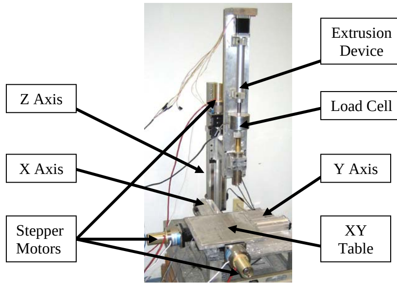
Figure 1: Picture of FEF experimental setup.
