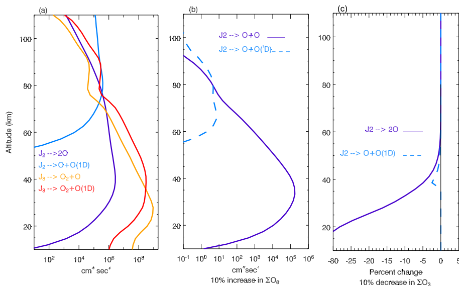
Fig. A2. (a) Vertical profiles of CHEM2D J_2 and J_3 photolysis terms for production of atomic oxygen in both ground state and excited state ( \text{O}(^1\text{D}) ) for March conditions at 30^\circ\text{N} ; (b) the absolute reduction in J_2 from (a) for an imposed 10% increase in overhead column ozone at each model vertical level; (c) as in (b) but for the percentage reduction in J_2 .
