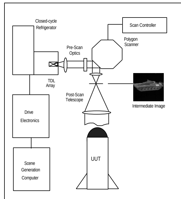
Figure 1. Projector schematic
