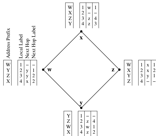
Figure 8. Label-Swapping with Addresses
