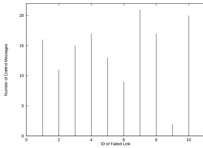
Figure 6: MIP's control overhead for link failures.
