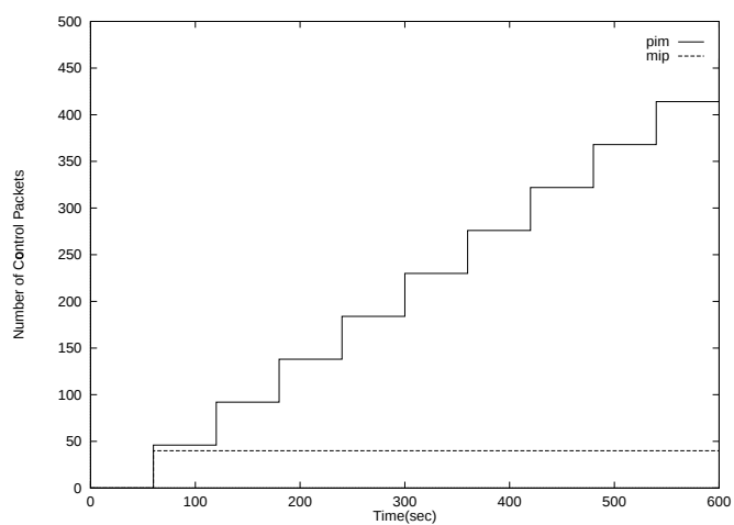
Figure 5: Control overhead of MIP vs. PIM.
