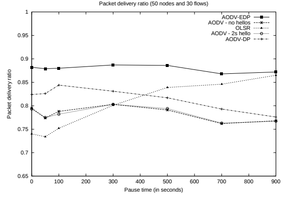
Fig. 4. Packet delivery ratio for 50 nodes and 30 flows (120 packets/s)
