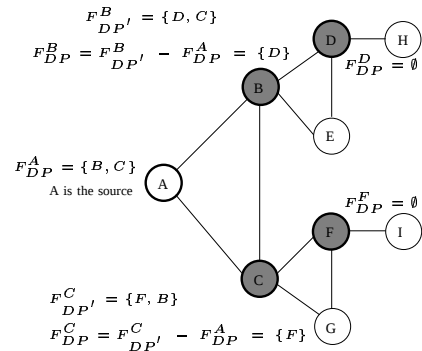
Fig. 1. Example where original DP fails (node A is the source). Modified DP determines the correct set of forwarding nodes: A selects B and C as forwarder nodes; B chooses D and C as forwarder nodes, but dismiss C because it is in the sender's forwarder list; C chooses F and B , but dismiss B because it is in the sender's forwarder list.
