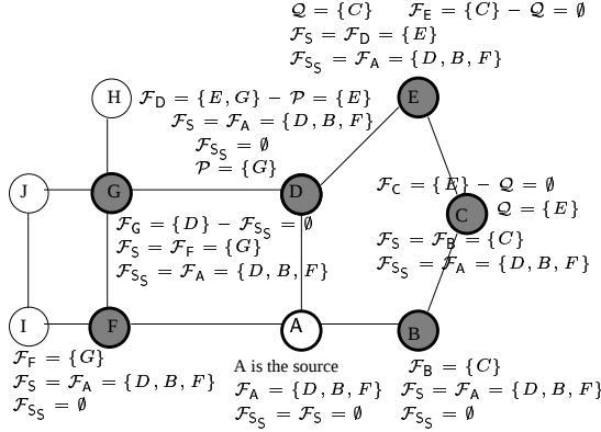
Fig. 2. Node A is the source. The knowledge about the second to previous forwarder list ( \mathcal{F}_A ) allows nodes E and C to exclude each other from their forwarder list, and node G to exclude node D. Node D reduces the size of its forwarder list by using the information provided by the set \mathcal{P} .
