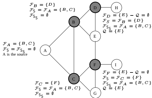
Fig. 3. Node A is the source. Nodes B, C, D, F are the only nodes chosen as forwarders for this network.
