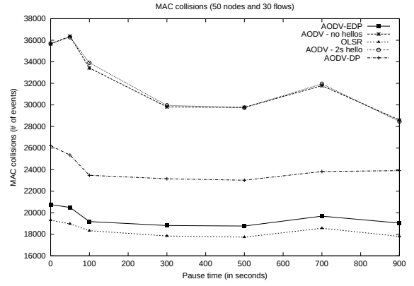
Fig. 7. MAC collisions for 50 nodes and 30 flows (120 packets/s)
