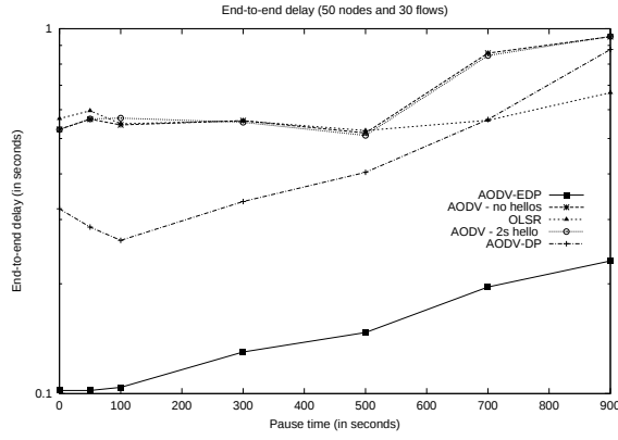
Fig. 5. End-to-end delay for 50 nodes and 30 flows (120 packets/s)
