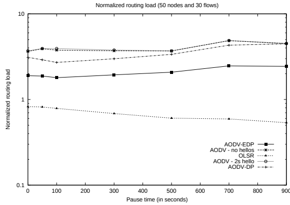
Fig. 6. Routing load for 50 nodes and 30 flows (120 packets/s)
