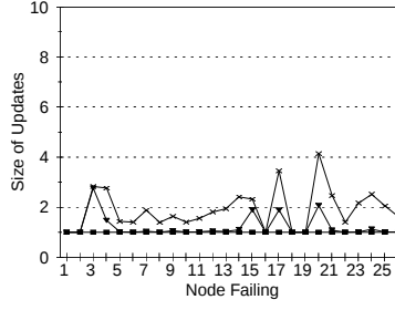
Fig. 16. Size of updates for node failures
