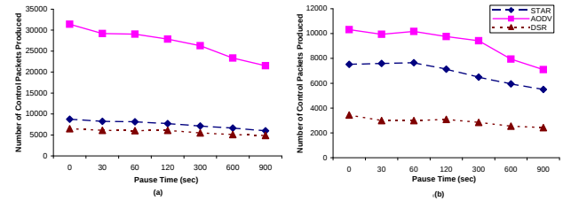
Fig. 2. Control Overhead in Scenario 1 for (a) 60 (b) 20 Data Flows
