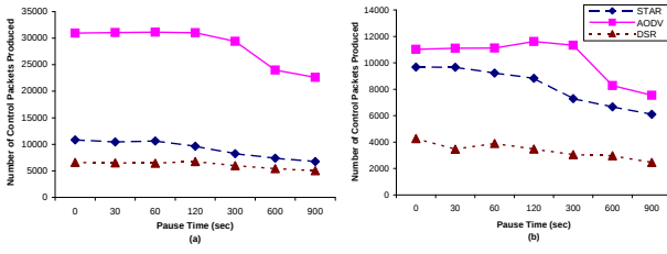
Fig. 11. Control Overhead in Scenario 4 for (a)60 (b)20 Data Flows
