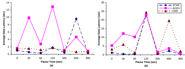
Fig. 15. Data Latency in Scenario 5 for (a) 60 (b) 20 Data Flows
