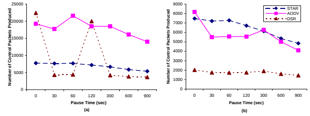
Fig. 5. Control Overhead in Scenario 2 for (a) 60 (b) 20 Data Flows
