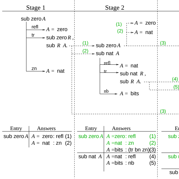
Figure 4.1: Staged computation
