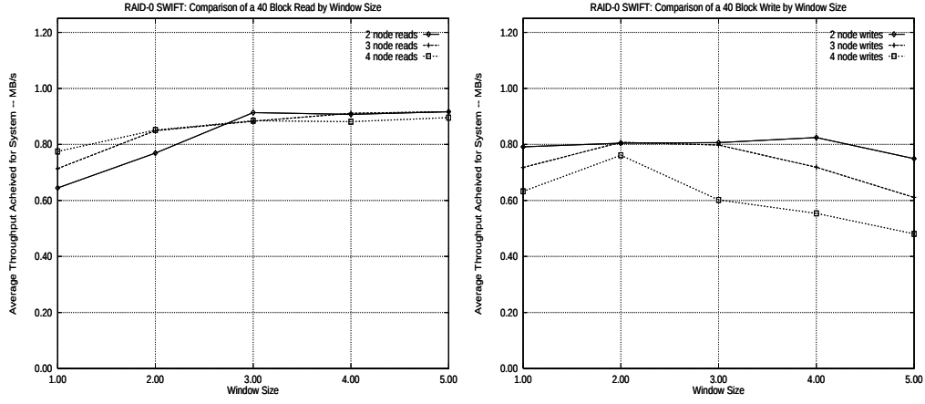
Figure 2: RAID-0 adaptive prototype performance.
