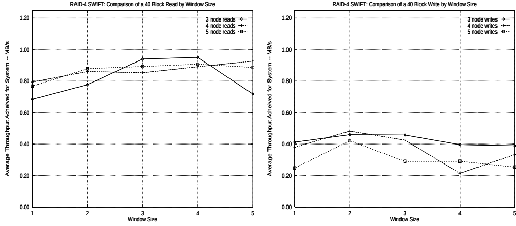
Figure 3: RAID-4 adaptive prototype performance.
