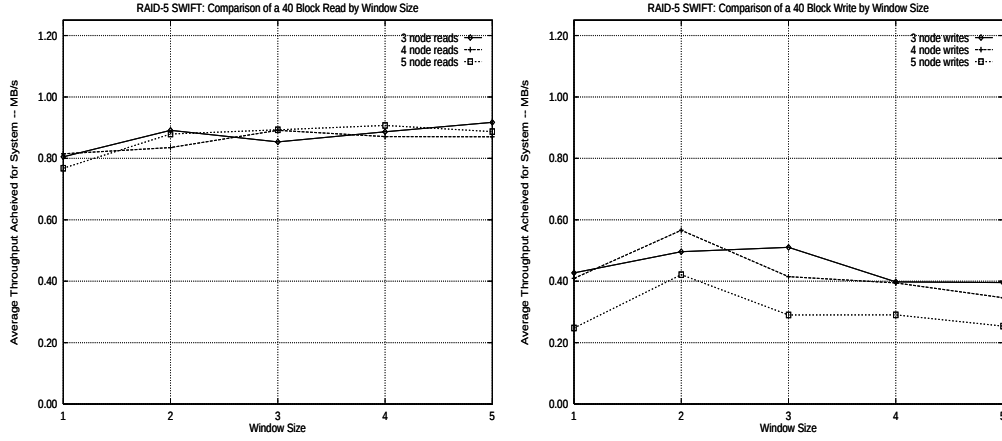
Figure 4: RAID-5 adaptive prototype performance.
