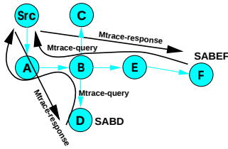
Figure 5: Routers D and F send an MTRACE along the reverse path to the source. The source's router returns the recorded path-string via unicast.
