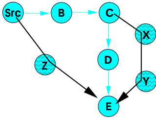
Figure 3: Measuring multicast distances incorrectly with unicast propagation delay. Multicast paths are shown with gray arrows.
