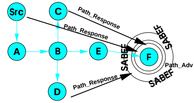
Figure 6: Path advertisement by the host attached to router F via ERS. The source, and hosts attached to routers C and D answer in this example.
