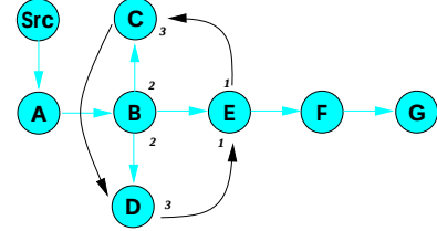
Figure 2: Possible looping from using hop counts.
