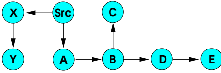
Figure 4: For a host attached at router E, host attached to router D are directly acceptable; hosts at router C are indirectly acceptable; and hosts at router X are unacceptable.
