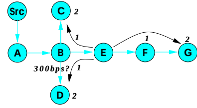
Figure 1: Problems with using hop count.
