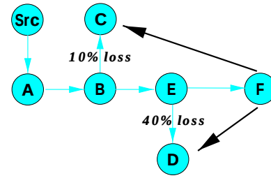
Figure 8: Because router D is behind a lossy link, hosts at F choose retransmitters at C.
