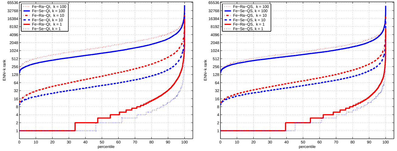
Figure 6: Comparison of the two methods for choosing training triples: sampling them from the set of all possible triples vs. choosing them from a selective subset of triples. We plot ENN-k ranks vs. percentile, for 256-dimensional embeddings, for k = 1, 10, 100 . On the left we show query-insensitive embeddings, on the right we show query-sensitive embeddings. In all cases, and for all percentiles, choosing triples selectively leads to better results.
