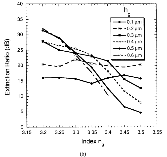
Fig. 3. (a) The coupling length and (b) the extinction ratio as a function of gap layer index for different thicknesses of the gap layer.
