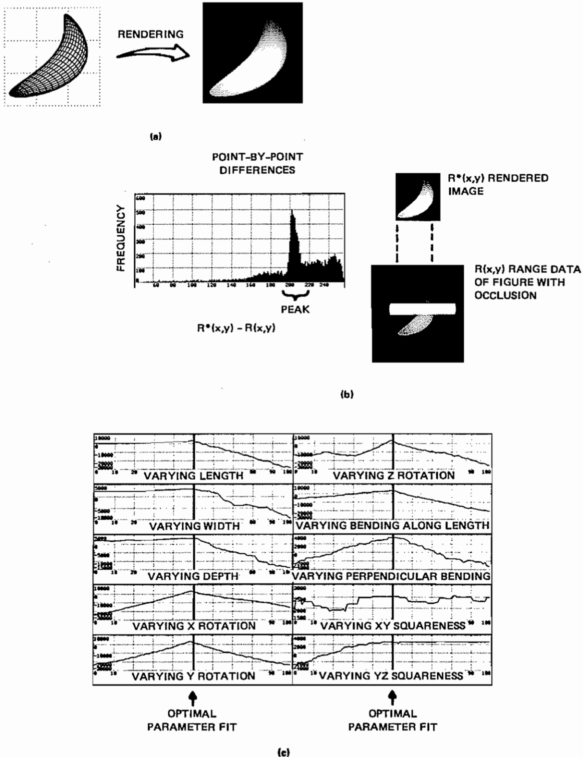
Figure 6: Finding the best fitting part descriptor. (a) We take a 3-D SuperSketch part with the hypothesized parameters (e.g., orientation, length, squareness), render it using known sensor characteristics to produce a predicted image R^*(x,y) . (b) We then histogram point-by-point differences (i.e., R^*(x,y) - R(x,y) ) between the R^* and the range data R(x,y) ; the size of the largest peak is used to calculate our goodness of fit measure. (c) The fit between these range data and a 3-D part model as the parameters of the 3-D part are varied; the correct fit occurs at the center of each graph.
