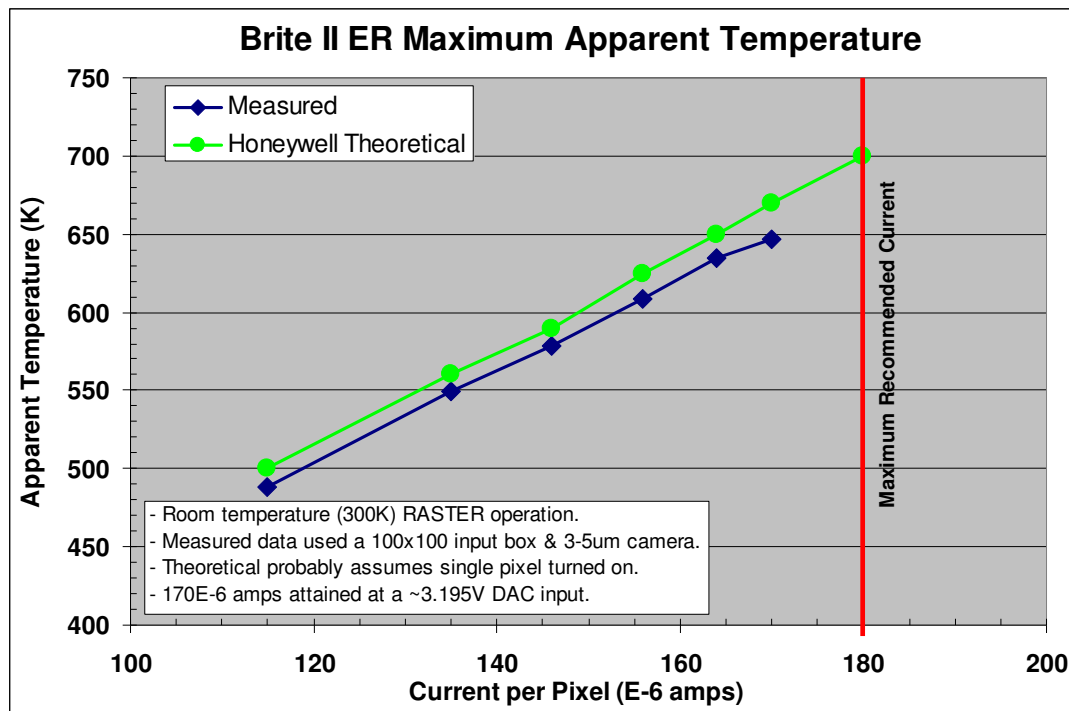
Figure 6 – BRITE II ER Array Maximum Apparent Temperature
