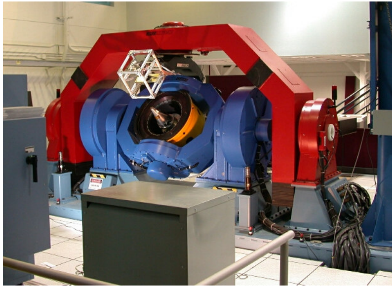
Figure 12 – FMS Table in the AMRDEC ASC
