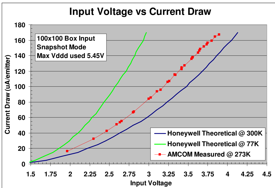
Figure 7 – BRITE II ER Extended Voltage Range Performance
