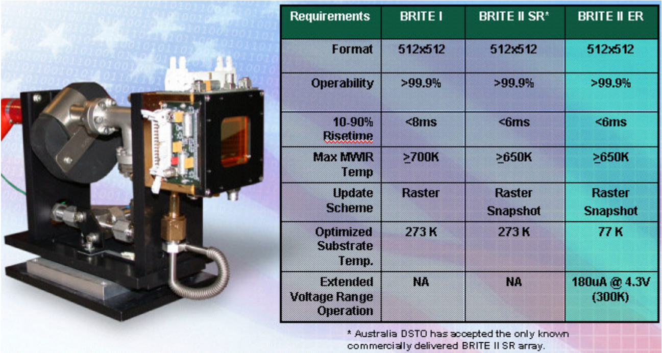
Figure 2 – BRITE II SR and ER Array Requirements
