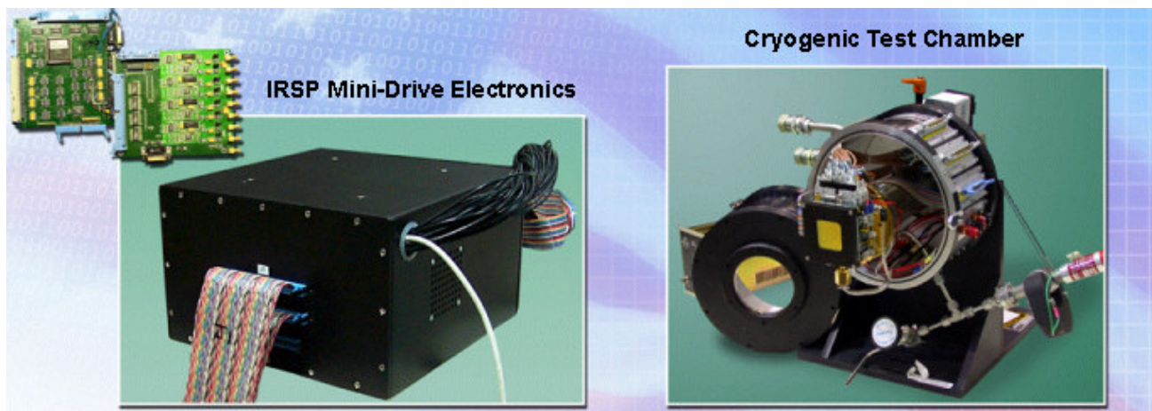
Figure 3 – ASC Emitter Array Drive Electronics and Cryogenic Test Chamber
