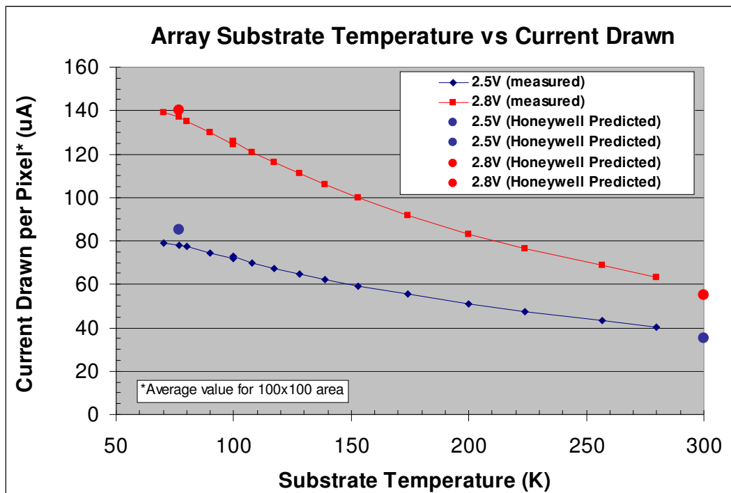
Figure 10 – BRITE II ER Array Cryogenic Operation Performance
