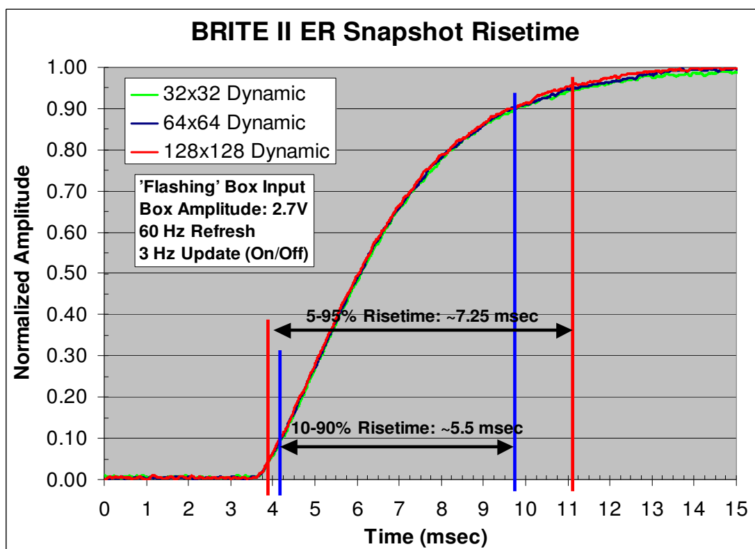
Figure 5 – BRITE II ER Emitter Array Risetime Measurement (Snapshot Mode)
