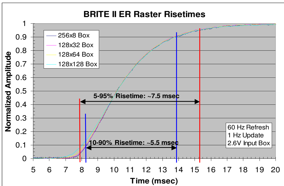
Figure 4 – BRITE II ER Emitter Array Risetime Measurement (Raster Mode)
