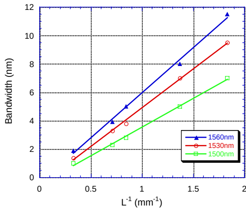
Fig. 27 Experimental (points) and theoretical (lines) coupler length dependence of the bandwidth.
