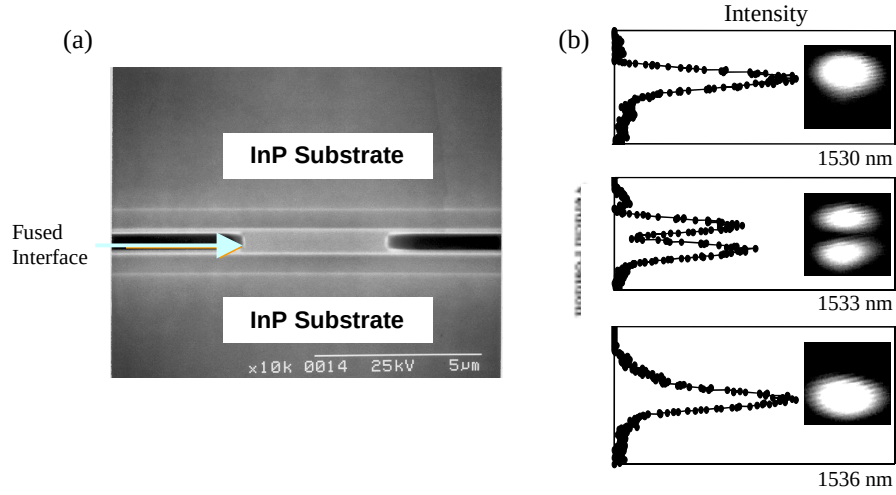
Figure 12 (a) The stained etched SEM picture of a fused vertical coupler. (b) Photograph of the near field pattern at 1530, 1533 and 1536 nm. The width of the ridge is 3 \mu\text{m} , and the distance between upper and lower waveguides is 1.1 \mu\text{m} .
