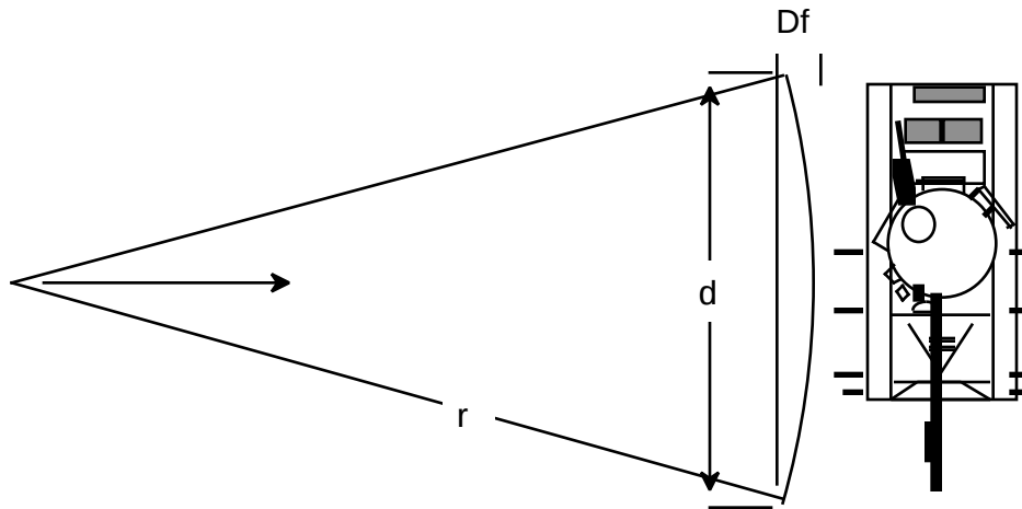
Figure 8. Phase variation of the incident wave front over the target extent.
