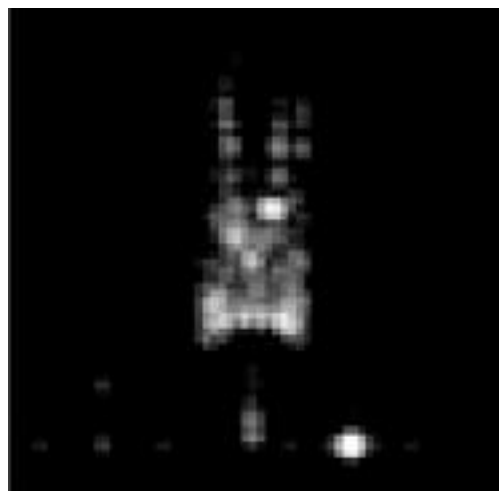
Figure 8. Incoherent sum of the 64 ISAR images measured from 4.5^\circ to 5.5^\circ in 0.015^\circ increments.
