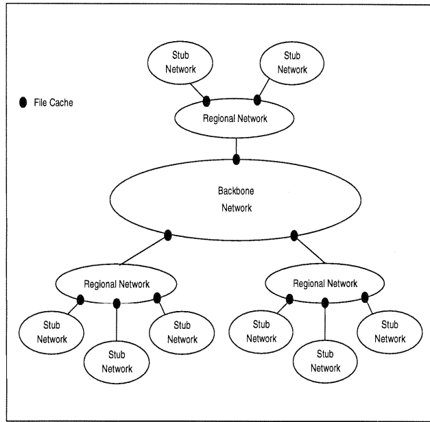
Figure 7: Topology-Based Cache Organization
