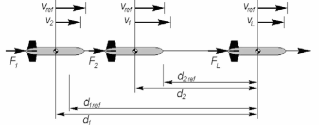
Fig. 2. Algorithm applied to 1D formation.
