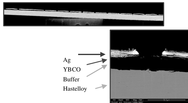
Figure 2. Cross-sectional views of striped YBCO conductor.
