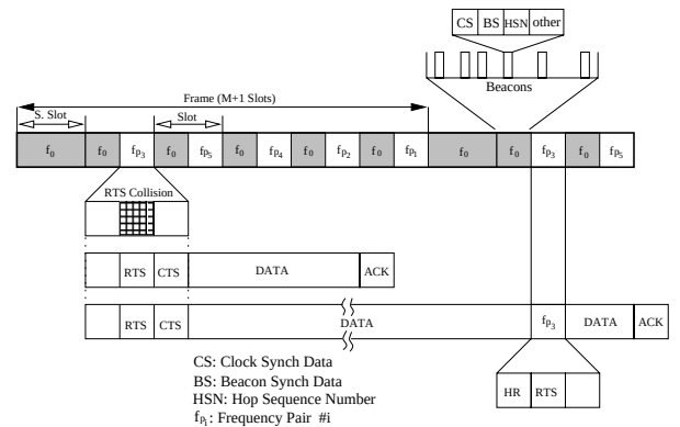
Figure 2: Structure of HRMA slot and frame
