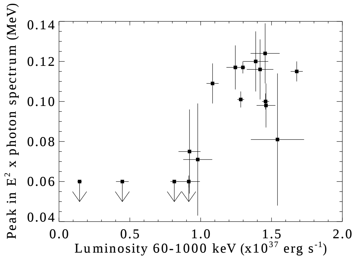
Figure 7: Peak in luminosity per decade versus luminosity between 60 and 1000 keV for the model fits of all the observations, as in Table 3.
