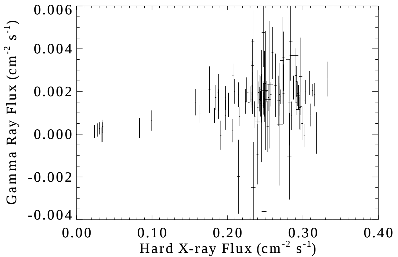
Figure 9: Flux in the 0.4-1.5 MeV band versus the flux in the 0.06-0.4 MeV band for each day of data. These bands are nearly identical to those in the compilation of Bassani et al. (1989).
