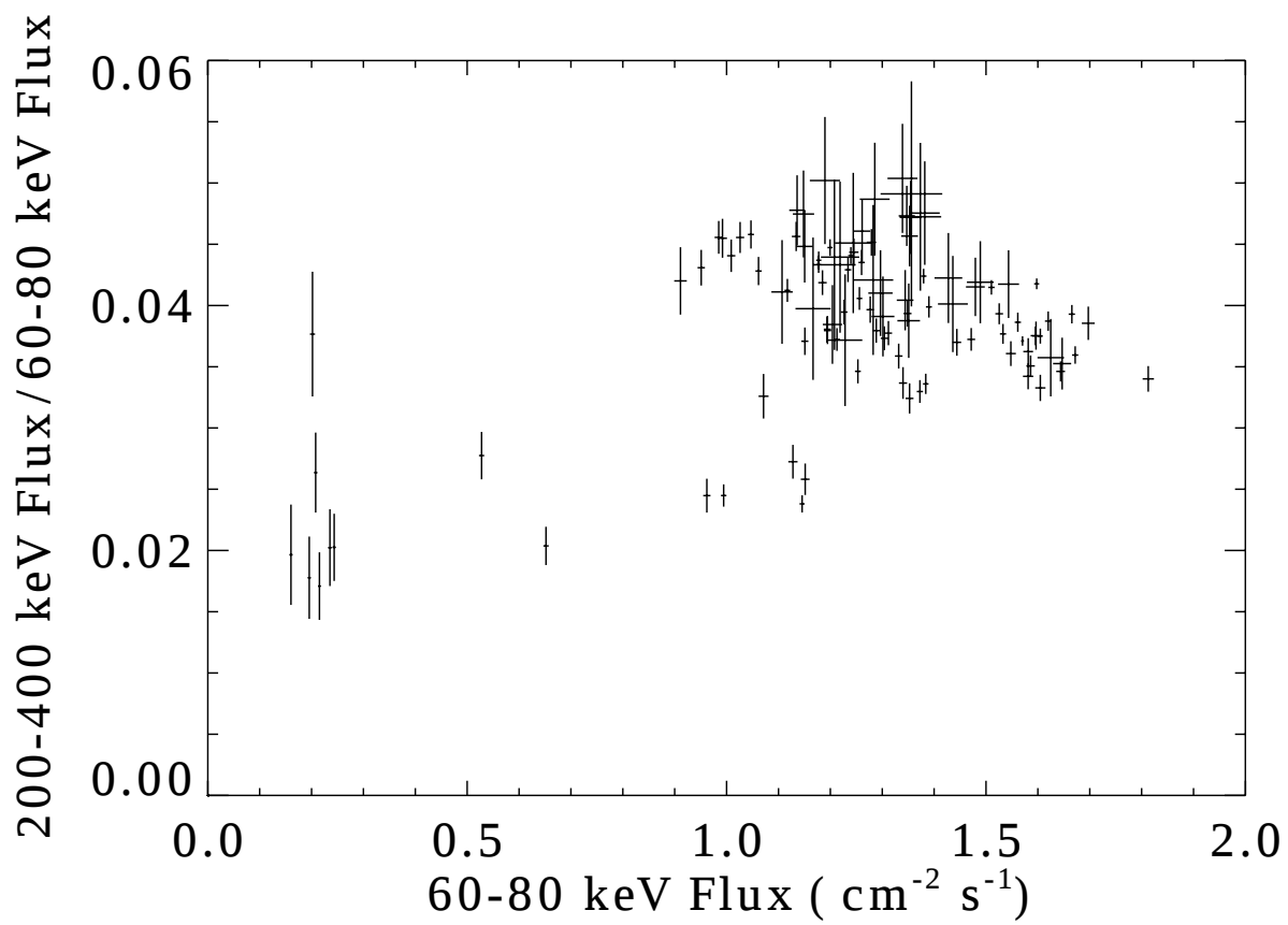
Figure 10: Ratio of the flux in the 200-400 keV band over the flux in the 60-80 keV band versus the flux in the 60-80 keV band for each day of data.
