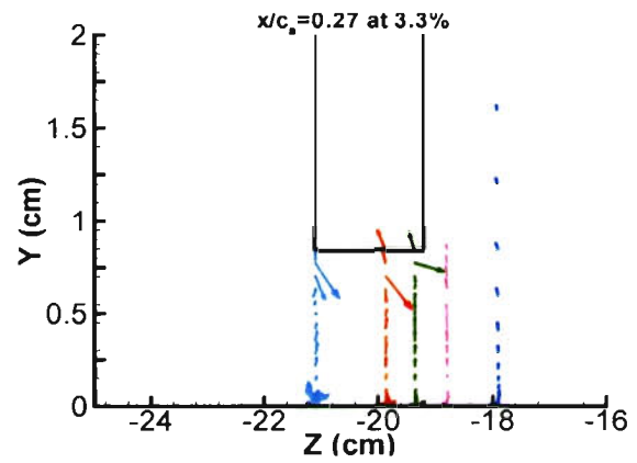
(l) x/c_a = 0.27 t/c = 3.30\%
