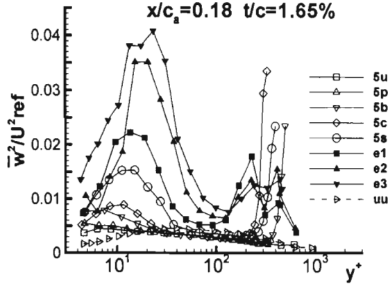
(a) x/c_a = 0.18 t/c = 1.65\%
