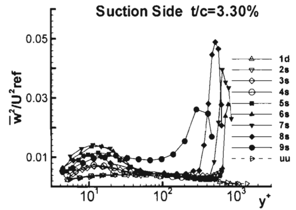
(f) Suction side t/c = 3.30\%
