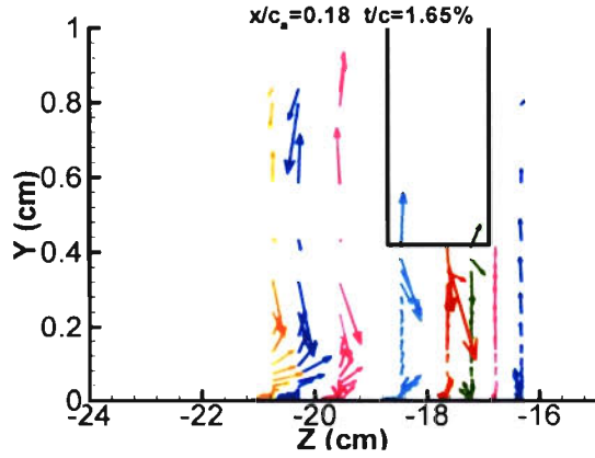
(i) x/c_a = 0.18 t/c = 1.65\%
