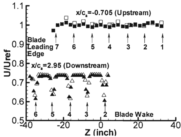
Figure 3.3: Velocities at tunnel half height upstream ( x/c_a = -0.705 ) and downstream ( x/c_a = 2.95 ) of blade row for stationary wall experiments in bed co-ordinates; arrows show location of given blade number; for this study: \square , x/c_a = -0.705 ; \triangle , x/c_a = 2.95 ; From Kuhl (2001): \blacksquare , x/c_a = -0.705 ; \blacktriangle , x/c_a = 2.95 .
