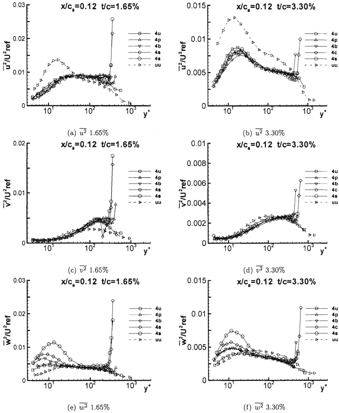
Figure F.4: Reynolds normal stresses \overline{u^2}/U^2_{ref} , \overline{v^2}/U^2_{ref} , and \overline{w^2}/U^2_{ref} at x/c_a = 0.12 for both 1.65% and 3.30% in chord coordinate system
