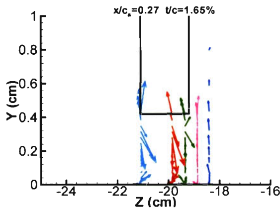
(k) x/c_a = 0.27 t/c = 1.65\%
