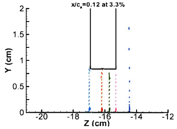
(h) x/c_a = 0.12 t/c = 3.30\%
