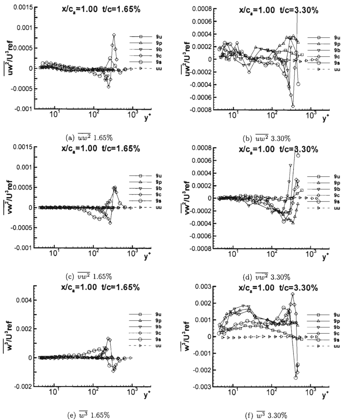
Figure G.27: Triple products \overline{uw^2}/U^3_{ref} , \overline{vw^2}/U^3_{ref} , and \overline{w^3}/U^3_{ref} at x/c_a = 1.00 for both 1.65% and 3.30% in chord coordinate system
