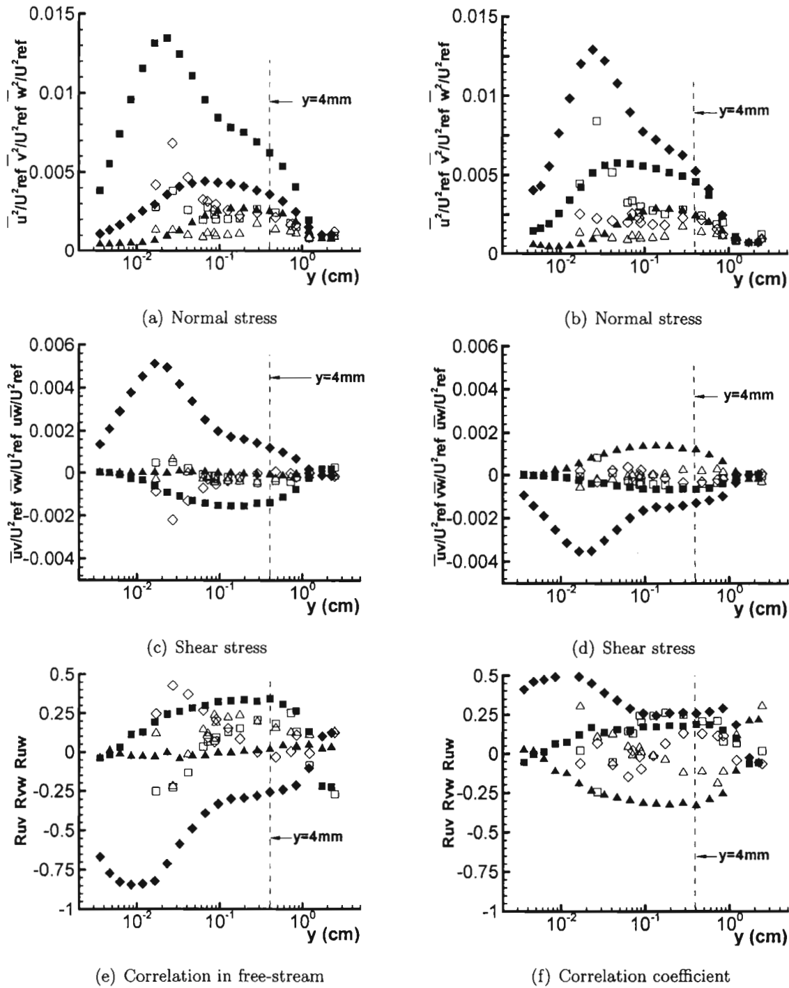
Figure 4.12: Reynolds stress profile uu at x/c_a = -0.33 with 3.30% tip gap for both free-stream and bed coordinate systems: (a), (c), and (e) in the free-stream coordinate system; (b), (d), and (f) in the bed coordinate system. For moving wall: □, \overline{u^2} , \overline{uv} , and R_{uv} ; △, \overline{v^2} , \overline{vw} , and R_{vw} ; ◇, \overline{w^2} , \overline{uw} , and R_{uw} . For stationary wall: ■, \overline{u^2} , \overline{uv} , and R_{uv} ; ▲, \overline{v^2} , \overline{vw} , and R_{vw} ; ◆, \overline{w^2} , \overline{uw} , and R_{uw} .
