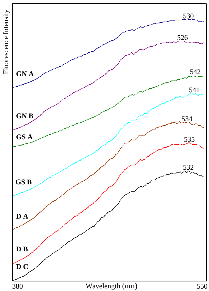
Figure 6. Fluorescence emission spectra of the humic acids isolated from the seven control greenhouse soils.
