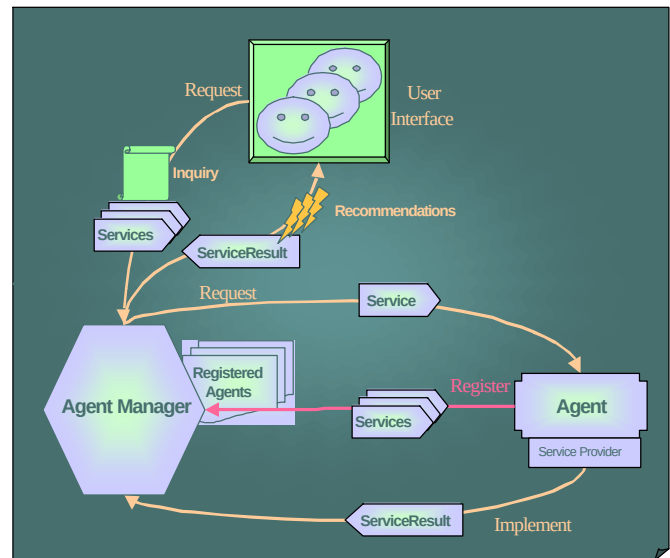
Figure 3. User Request
