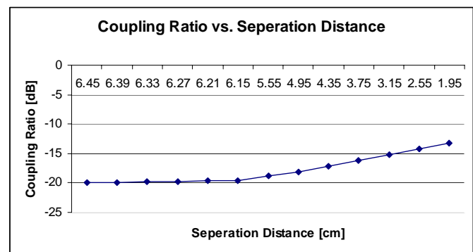
Figure 8. Coupling ratio between elements vs. separation distance.
