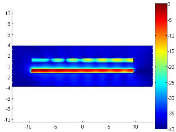
Figure 7. Normal fields in cavity for driven lower element and passive upper element.
