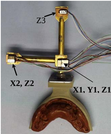
Figure 4. Six-Axis Bitebar
