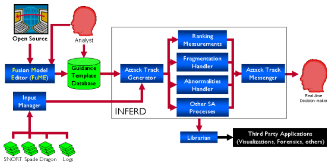
Figure 4. ECCARS Architecture
