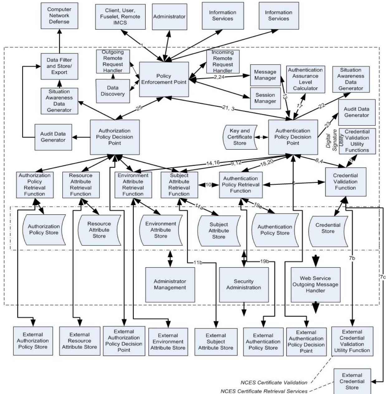
Figure 6 - NCES Thick Client Authentication
