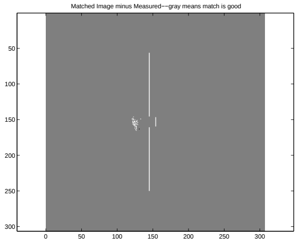
Fig. 10. Combining pose estimates with the CAD model, a predicted image is calculated and subtracted from the measured image.
