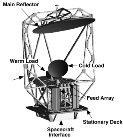
Fig. 1. Relevant components of the WindSat instrument involved in radiometric calibration.
