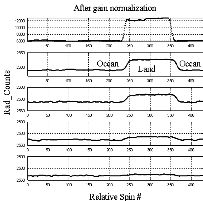
Fig. 23. Time series of rad_counts for 10.7-GHz H-pol during rev-2611. Upper panel is main reflector looking forward at the right-hand edge of swath. Second panel (from top) is the azimuth corresponding to the cold-sky reflector sweet-spot minus 16^\circ . Third panel is the azimuth corresponding to the sweet-spot minus 12^\circ . Fourth is the azimuth corresponding to the cold-load sweet-spot minus 8^\circ . The bottom panel is the azimuth corresponding to the cold-load sweet-spot.
