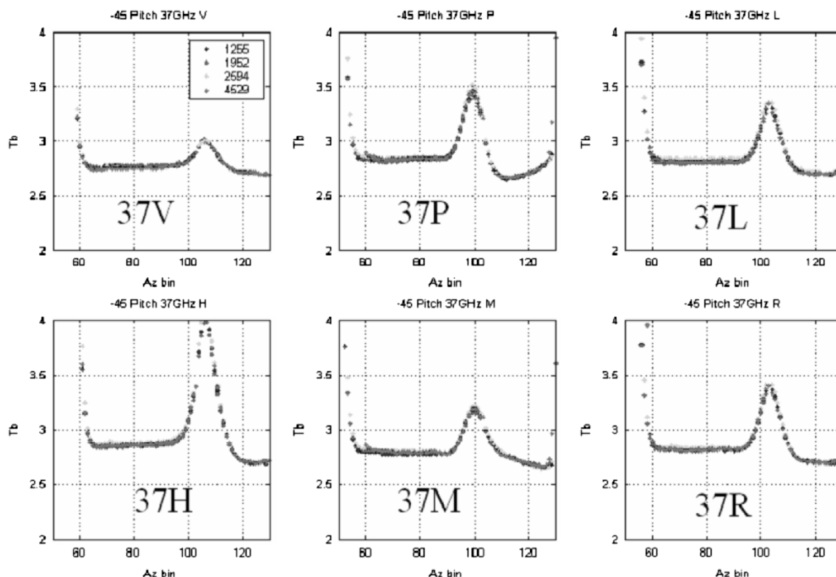
Fig. 21. Composite main and cold-sky reflector T_b s for aft look during -45^\circ pitch dwell for 37 GHz all polarizations for revs: 1255, 1952, 2594, and 4529. The X axis is azimuth bin number ( 2^\circ steps) where number 90 = 180^\circ .
