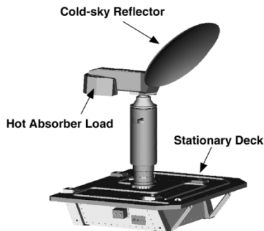
Fig. 3. WindSat calibration load nonrotating assembly.
