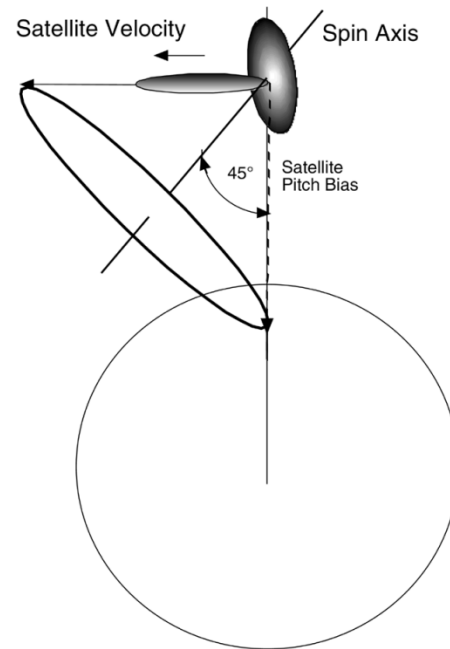
Fig. 10. WindSat conical-scanning measurement geometry during satellite pitch maneuver.
