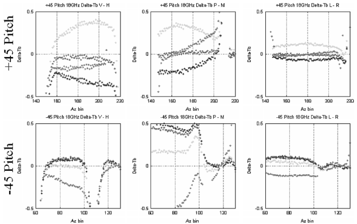
Fig. 34. Differential Tb for orthogonal channels (V-H, P-M, and L-R) during \pm 45^\circ pitch dwell for 18.7 GHz and for eight revs. The X axis is azimuth bin number ( 2^\circ steps).
