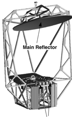
Fig. 2. WindSat antenna rotating assembly.
