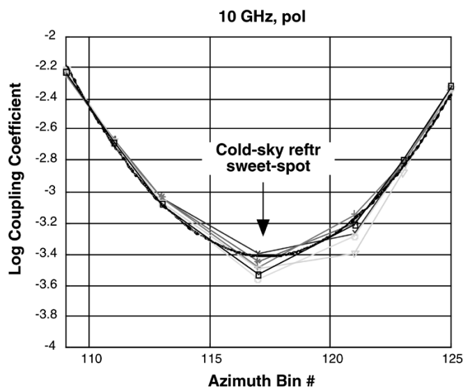
Fig. 25. Typical main reflector spillover coupling (six cases, 10.7 GHz, P-pol). The quadratic best fit curve is shown in bold black.
