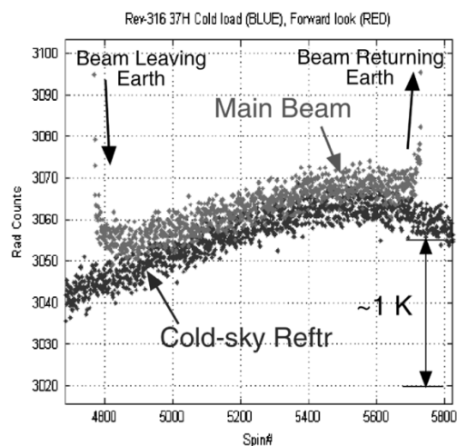
Fig. 15. Radiometer output (rad_counts) during pitch maneuver, rev-316, for main beam forward look (light gray) and cold-sky reflector (dark gray) for 37-GHz H-pol. The X axis is spin number (relative time).
