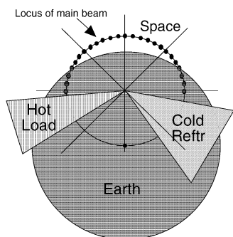
Fig. 11. Locus of main beam pointing into space during the positive 45^\circ pitch maneuver. Also shown are the azimuth blockage ranges for the hot and cold calibration loads.
