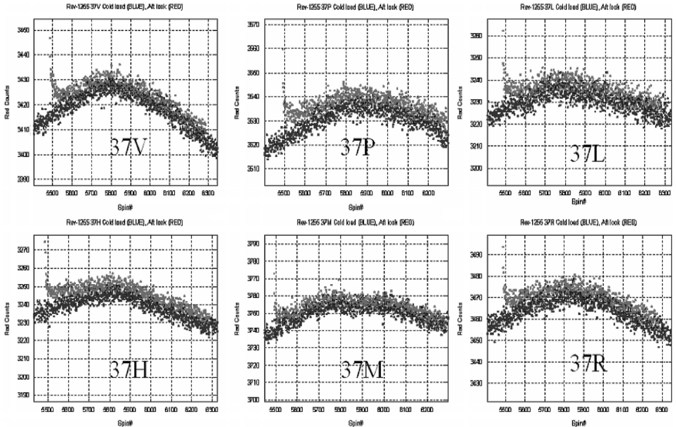
Fig. 19. Time series of radiometer output (rad_counts) during negative pitch maneuver, rev-1255, for main beam aft look (light gray) and cold-sky reflector (dark gray) for 37 GHz all polarizations. The X axis is spin number (relative time).
