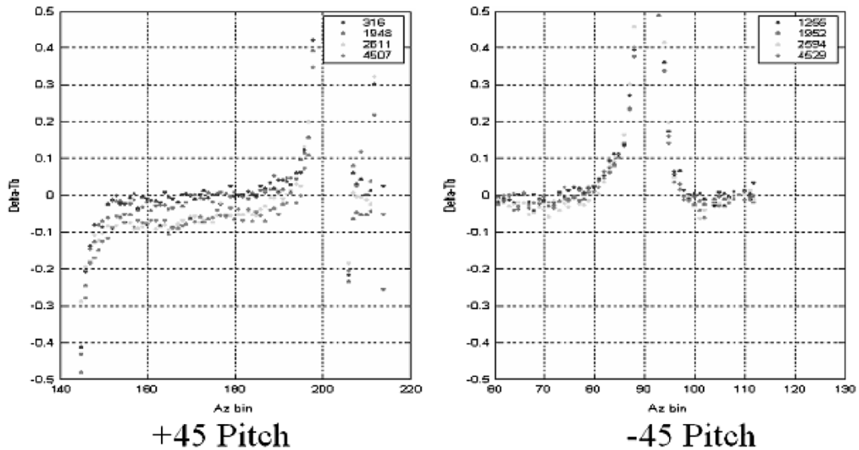
Fig. 28. Differential Tb for orthogonal (V-H) channels during \pm 45^\circ pitch dwell for 6.8 GHz and for eight revs (four positive and four negative pitch). The X axis is azimuth bin number ( 2^\circ steps).
