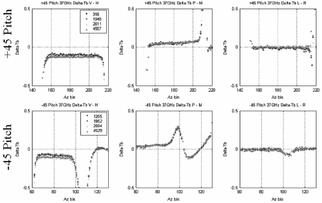
Fig. 22. Differential Tb for orthogonal channels (V-H, P-M, and L-R) during \pm 45^\circ pitch dwell for 37 GHz and for eight revs (four positive pitch in upper panels and four negative pitch in lower). The X axis is azimuth bin number ( 2^\circ steps).
