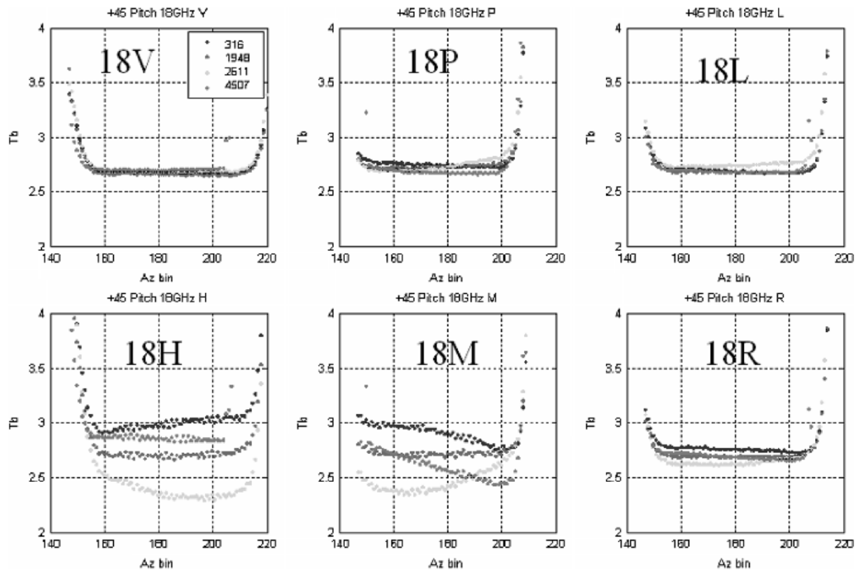
Fig. 32. Measured Tb for main reflector forward look during +45^\circ pitch dwell for 18.7 GHz all polarizations for revs: 316, 1948, 2611, and 4607. The X axis is azimuth bin number ( 2^\circ steps) where number 180 = 360^\circ and bin number < 180 view to the left side of the satellite subtrack and bin number > 180 view to the right.
