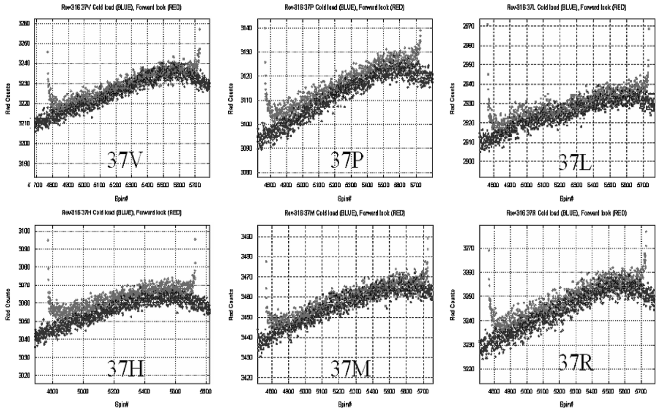
Fig. 16. Time series of radiometer output (rad_counts) during positive pitch maneuver, rev-316, for main beam forward look (light gray) and cold-sky reflector (dark gray) for 37 GHz all polarizations: V = vertical, H = horizontal, P = +45^\circ , M = -45^\circ , L = left-hand circular and R = right-hand circular. The X axis is spin number (relative time).
