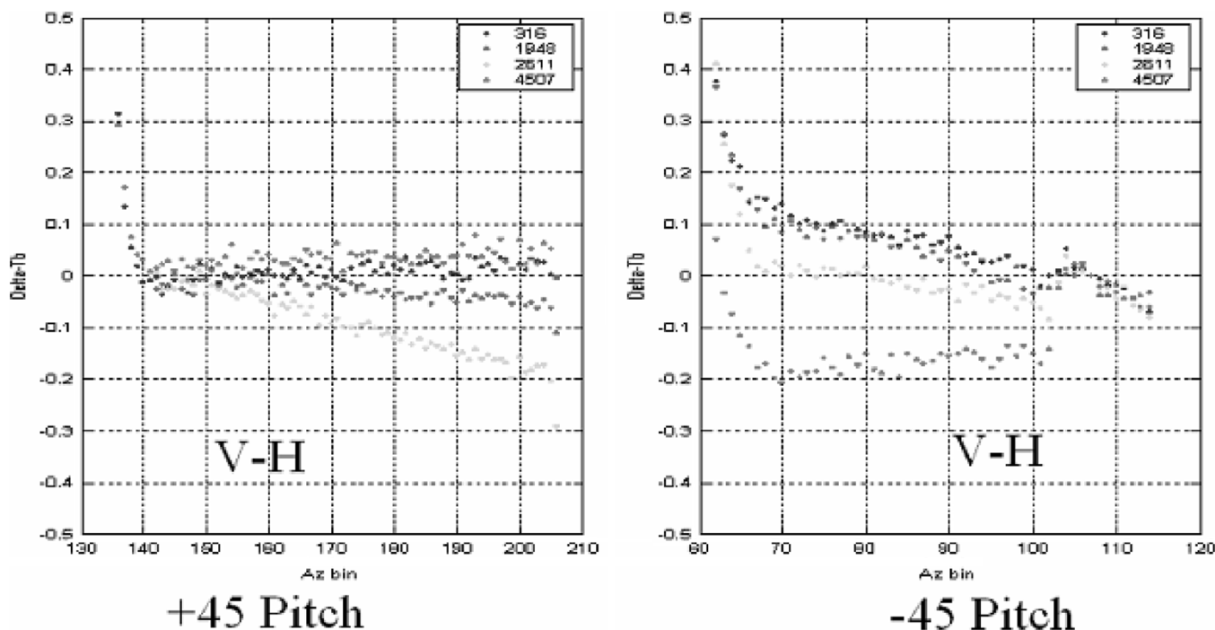
Fig. 37. Differential T_b for orthogonal channels (V-H) during \pm 45^\circ pitch dwell for 23 GHz and for eight revs. The X axis is azimuth bin number ( 2^\circ steps) where number 180 = 360^\circ and binnumber 90 = 180^\circ .
