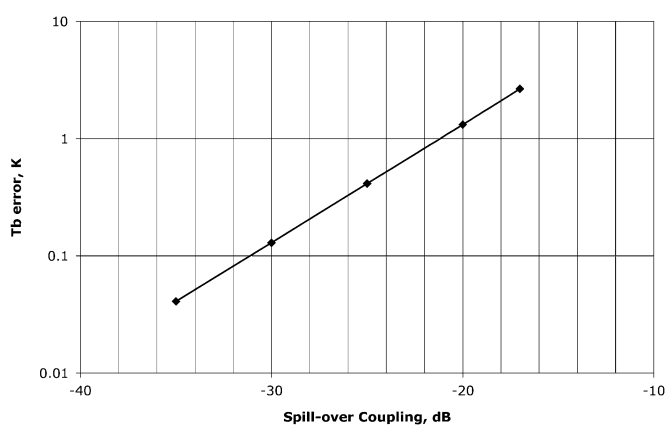
Fig. 26. Tb error introduced by main reflector spillover coupling for a typical ocean scene of 165 K.
