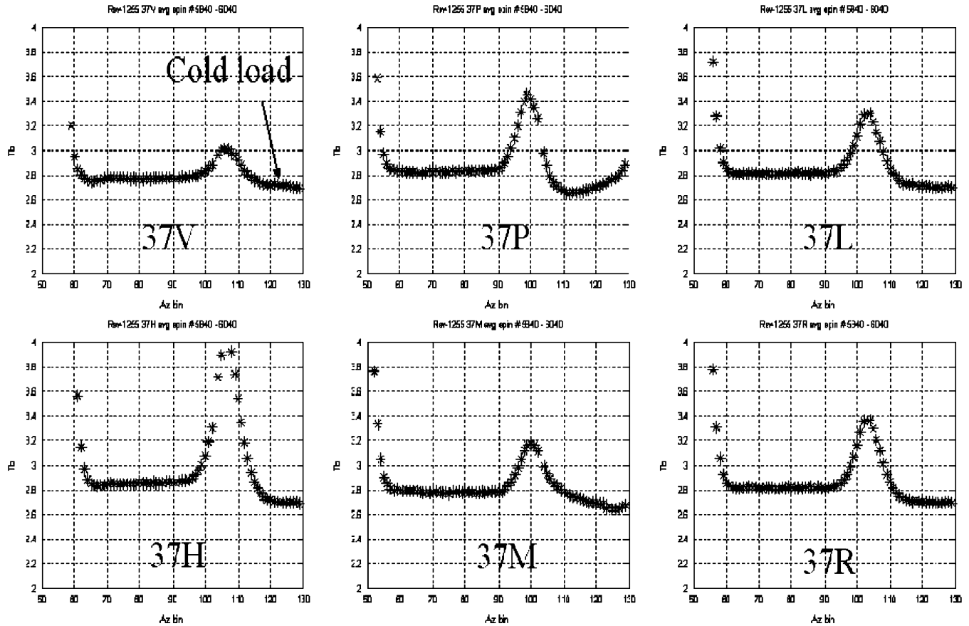
Fig. 20. Measured azimuthal distribution of main and cold-sky reflector T_b s (aft look) during -45^\circ pitch dwell, rev-1255, for 37 GHz all polarizations. The X axis is azimuth bin number ( 2^\circ steps) where number 90 is an azimuth of 180^\circ .
