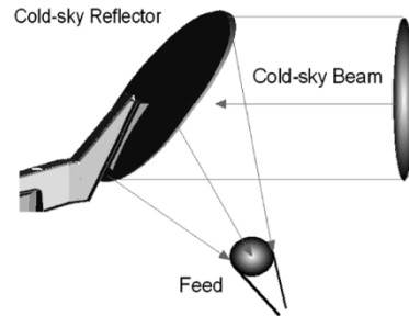
Fig. 5. WindSat cold-sky reflector (cold load) configuration. Eleven feeds sequentially move beneath the stationary reflector and form beams that view space.
