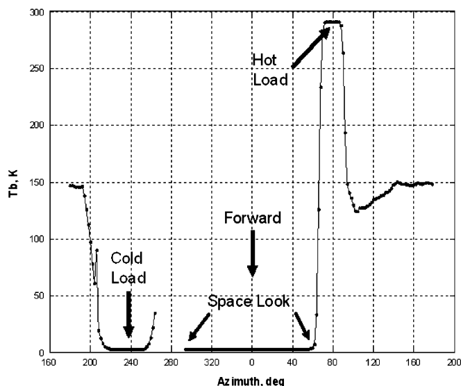
Fig. 12. Typical measured T_b (18 GHz), during a +45^\circ pitch maneuver. Forward measurement swath covers azimuth angles from approximately 290^\circ to 50^\circ (exact azimuth range is dependent upon individual feeds).
