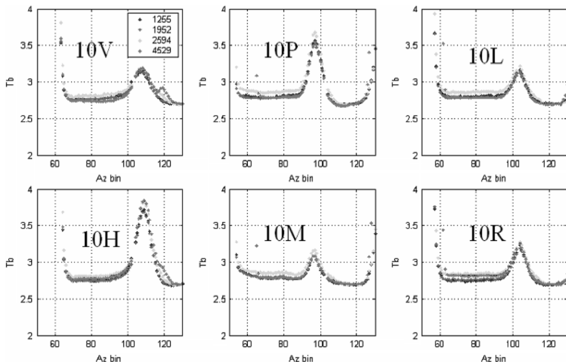
Fig. 30. Measured Tb for main and cold-sky reflectors for aft look during -45^\circ pitch dwell for 10.7 GHz all polarizations for revs: 1255, 1952, 2594, and 4529. The X axis is azimuth bin number ( 2^\circ steps) where number 90 = 180^\circ .
