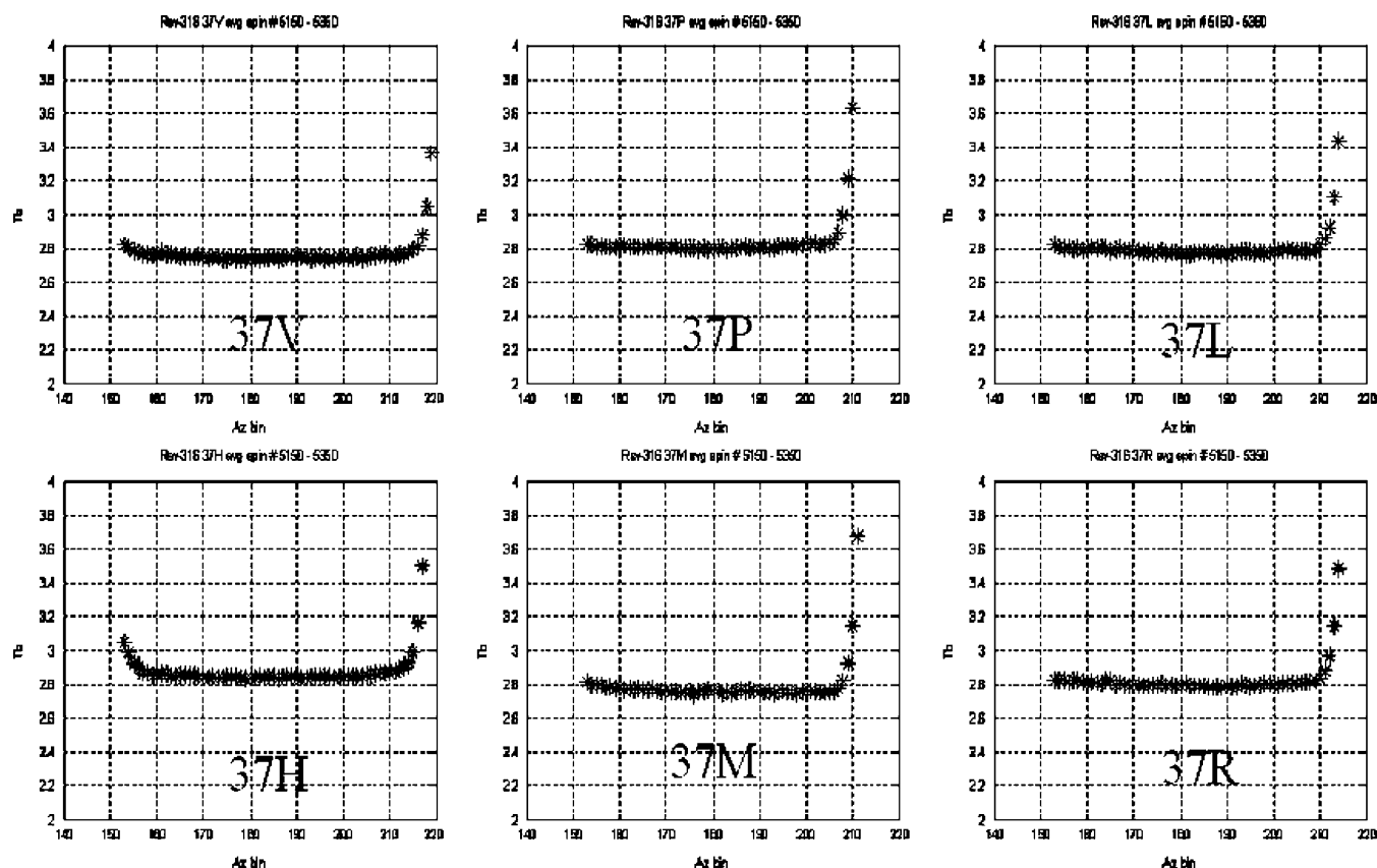
Fig. 17. Measured azimuthal distribution of main reflector Tb (forward look) during +45^\circ pitch dwell, rev-316, for 37 GHz all polarizations. The X axis is azimuth bin number ( 2^\circ steps) where number 180 = 360^\circ and bin number <180 view to the left side of the satellite subtrack and bin number >180 view to the right.
