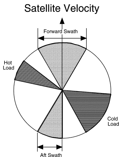
Fig. 8. Azimuthal distribution of WindSat measurement sectors.
