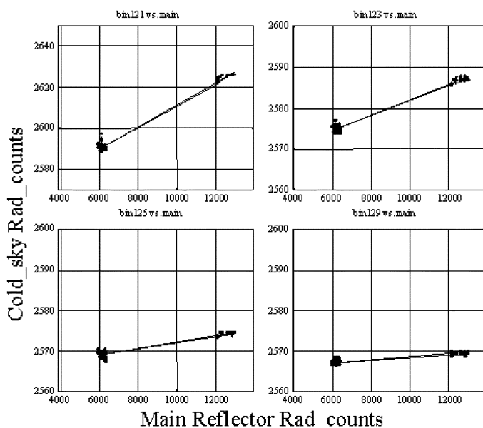
Fig. 24. Example of main reflector spillover determination over Australia, rev-2611. The slope of the linear regression line is the coupling coefficient. Upper left panel is the azimuth corresponding to the cold-sky reflector sweet-spot minus 16^\circ . Upper right is the azimuth corresponding to the sweet-spot minus 12^\circ . Lower left is the azimuth corresponding to the cold-load sweet-spot minus 8^\circ . The lower right is the azimuth corresponding to the cold-load sweet-spot.
