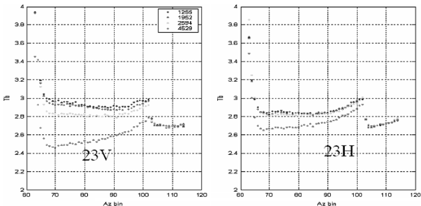
Fig. 36. Measured T_b for main reflector aft look during -45^\circ pitch dwell for 23 GHz for V-pol and H-pol for revs: 1255, 1952, 2594, and 4529. The X axis is azimuth bin number ( 2^\circ steps) where number 90 = 180^\circ .
