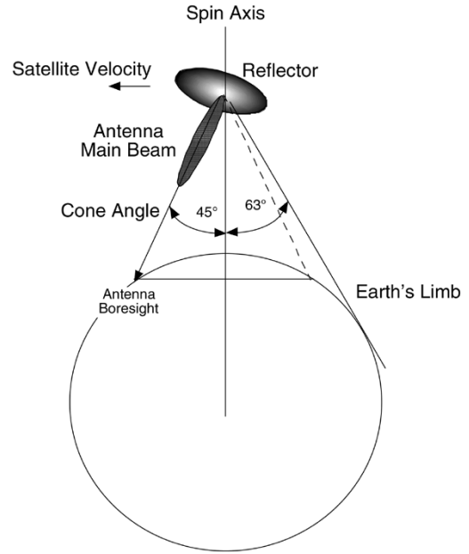
Fig. 9. WindSat normal conical-scanning measurement geometry.
