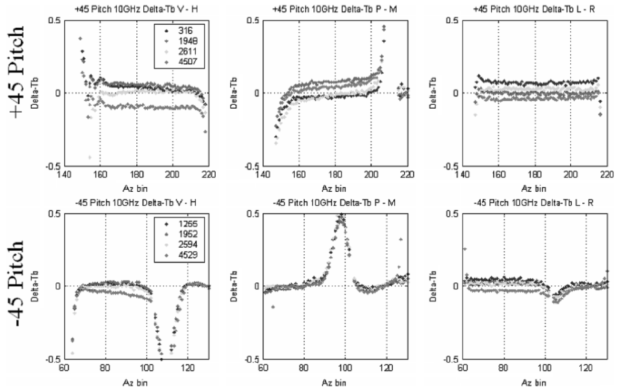
Fig. 31. Differential Tb for orthogonal channels (V-H, P-M, and L-R) during \pm 45^\circ pitch dwell for 10.7 GHz and for eight revs. The X axis is azimuth bin number ( 2^\circ steps) where number 180 = 360^\circ and binnumber 90 = 180^\circ .
