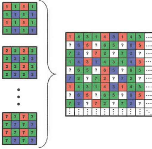
Figure 5. Fusion of 7 Bayer pattern low-resolution images with relative translational motion (the figures in the left side of the accolade) results in a high-resolution image ( \hat{Z} ) that does not follow a Bayer pattern (the figure in the right side of the accolade). The symbol “?” represents the high-resolution pixel values that were undetermined after the Shift-And-Add step (as a result of insufficient low-resolution frames).
