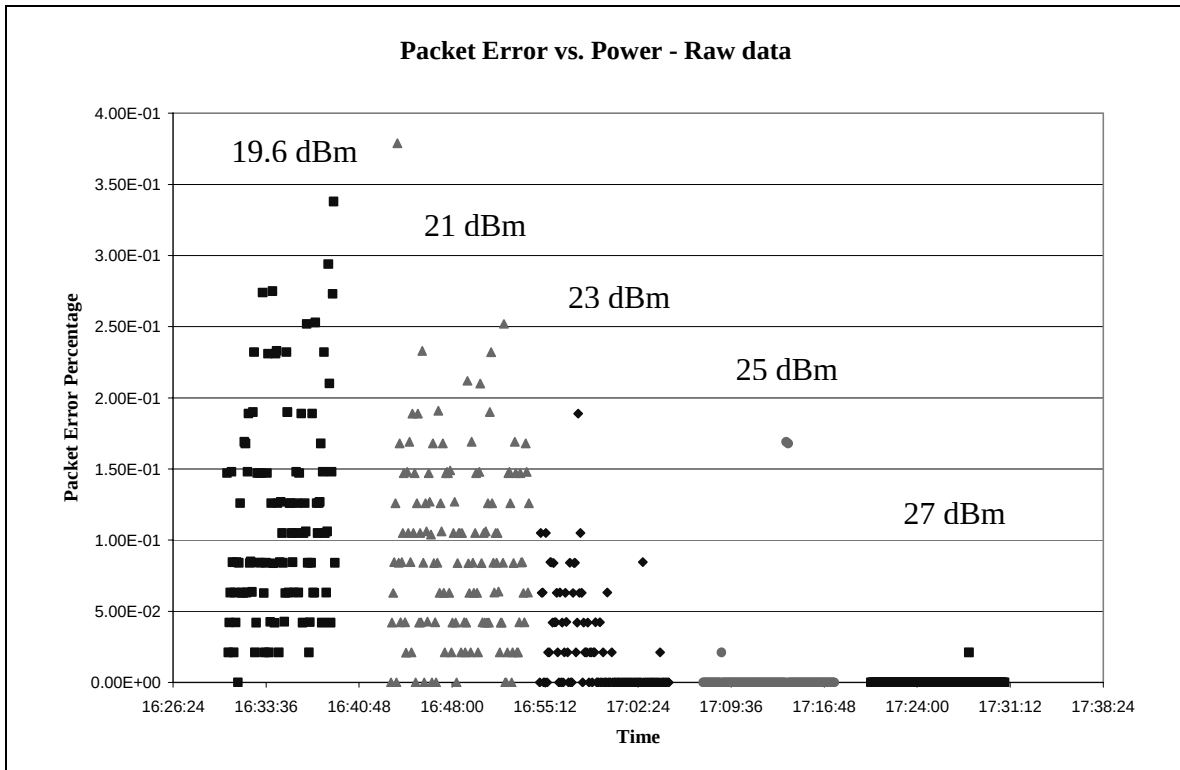
Figure 9: Raw packet error data for February 24 th , 2006
