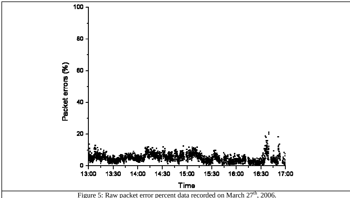
Figure 5: Raw packet error percent data recorded on March 27 th , 2006.
