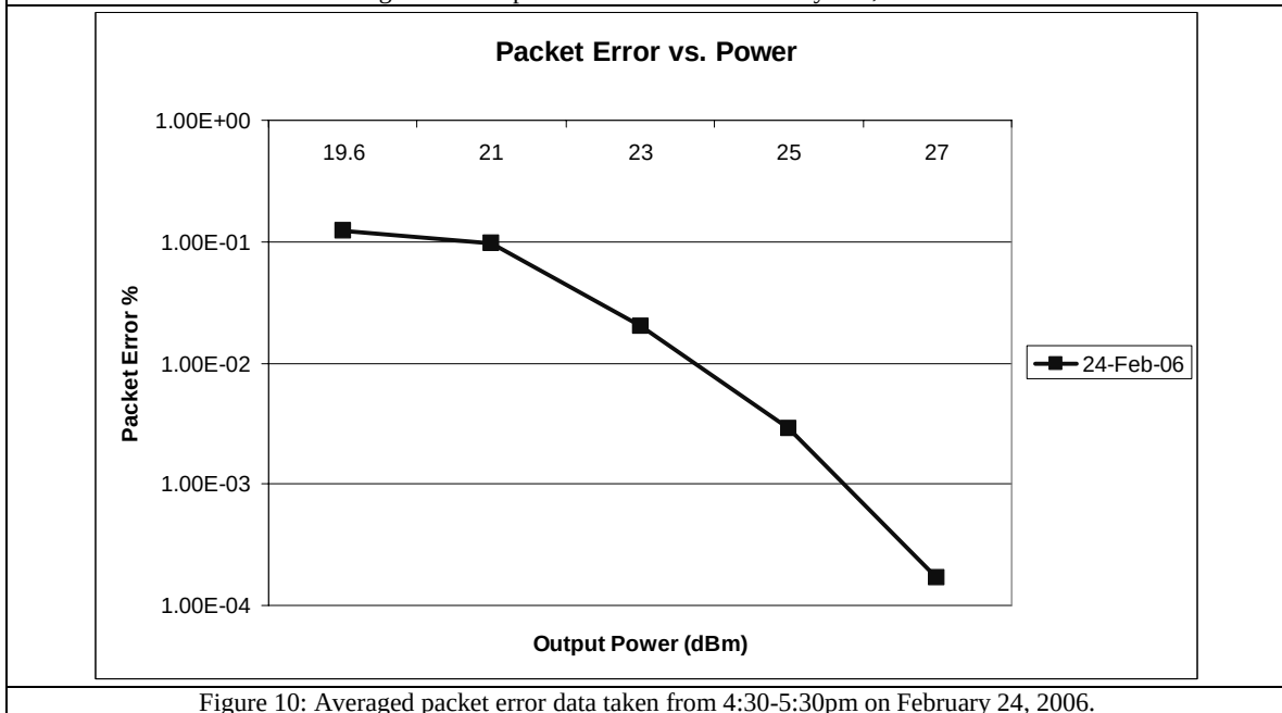
Figure 10: Averaged packet error data taken from 4:30-5:30pm on February 24, 2006.
