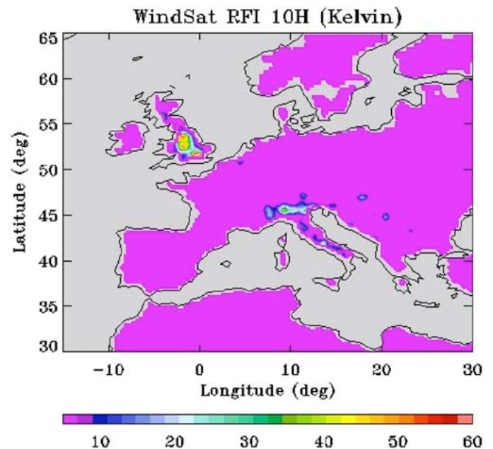
Fig. 6. WindSat X-band PCA-based RFI distribution for horizontal polarization over Europe.
