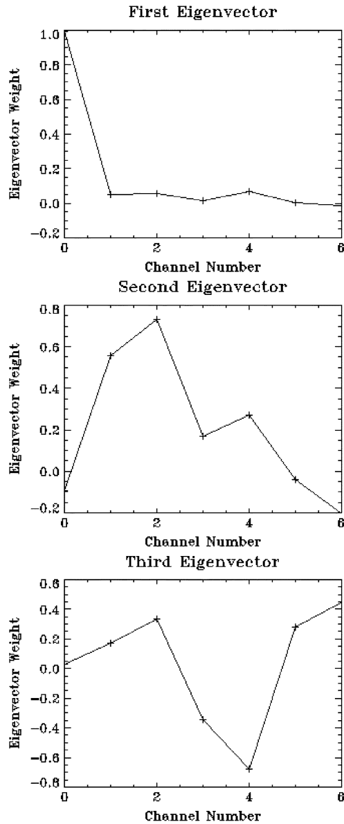
Fig. 4. Top three eigenvectors of WindSat RFI indices.
