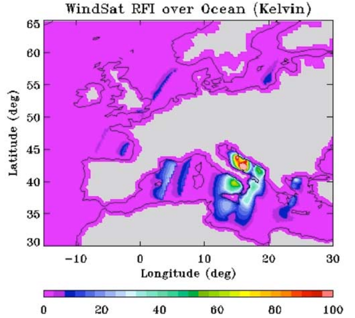
Fig. 7. WindSat X-band model difference-based RFI distribution for horizontal polarization over the Mediterranean Sea and North Sea.
