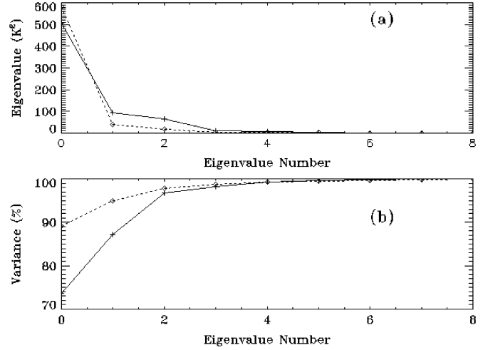
Fig. 1. Comparisons of WindSat and SMMR eigenvalues and variance. WindSat data are indicated by a solid line and SMMR by a dotted line.
