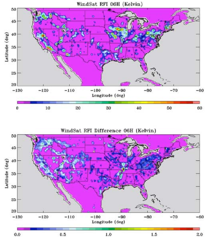
Fig. 5. WindSat C-band RFI distribution for horizontal polarization over the U.S. using (top panel) a PCA-based method and (bottom panel) the absolute difference between PCA-based and spectral difference methods (PCA minus Spectral Difference).
