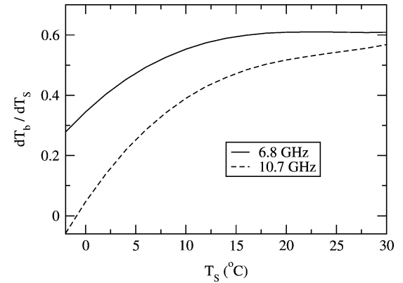
Fig. 8. Derivative of T_v with respect to T_S at 6.8 and 10.7 GHz calculated using the forward model.
