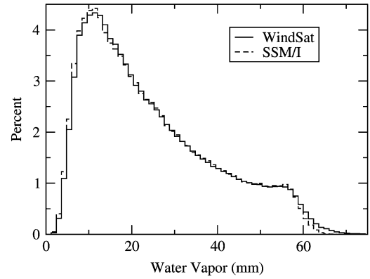
Fig. 3. Histograms of the WindSat and SSM/I water vapor retrievals for more than 33 million collocations.
