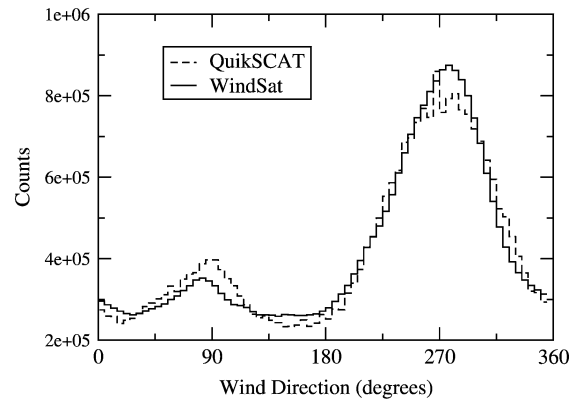
Fig. 11. Wind direction histograms for WindSat and QuikSCAT in 5^\circ bins for more than 29 million collocations.
