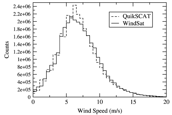
Fig. 10. Wind speed histograms for WindSat and QuikSCAT in 1-m/s bins for more than 29 million collocations.
