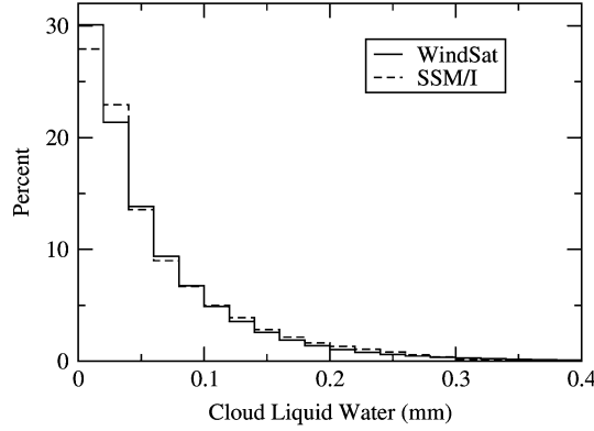
Fig. 5. Histograms of the WindSat and SSM/I cloud liquid water retrievals for more than 33 million collocations.
