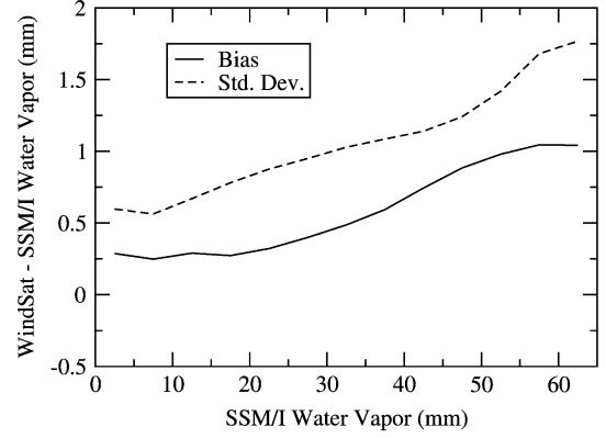
Fig. 2. Difference between the WindSat and SSM/I water vapor retrievals versus SSM/I water vapor.
