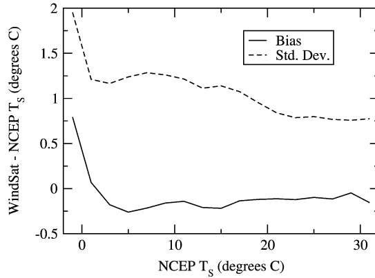
Fig. 6. Difference between the WindSat T_S retrievals and NCEP T_S results versus NCEP T_S .
