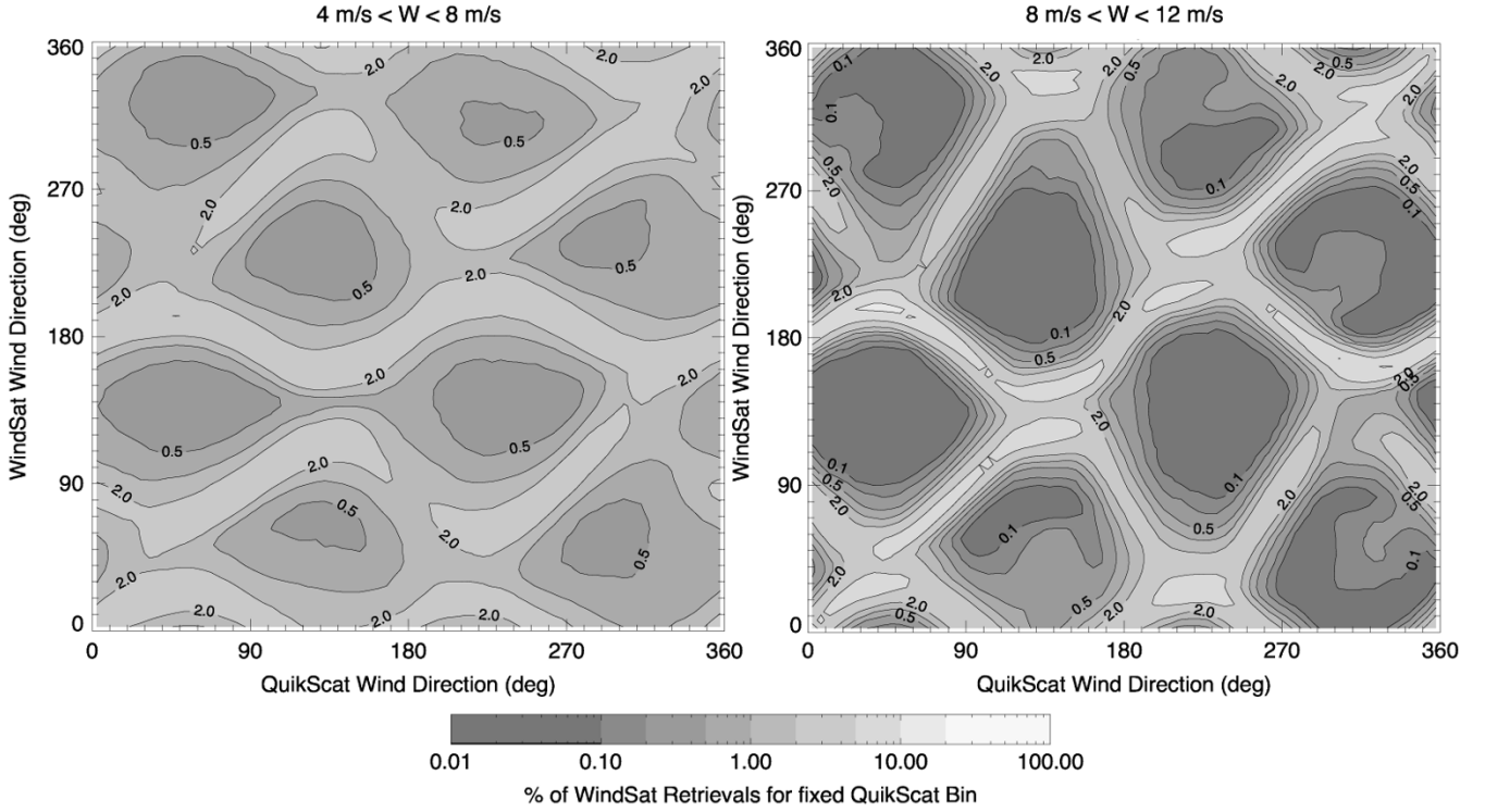
Fig. 18. Two-dimensional histogram of the ambiguities in 5^\circ \times 5^\circ bins of WindSat versus QuikSCAT wind direction relative to the WindSat look direction.
