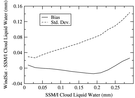
Fig. 4. Difference between the WindSat and SSM/I cloud liquid water retrievals versus SSM/I retrievals.
