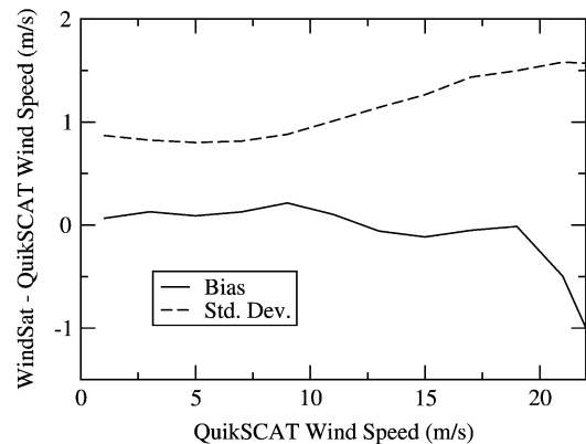
Fig. 12. Difference between WindSat and QuikSCAT retrieved wind speeds in 2-m/s wind speed bins.
