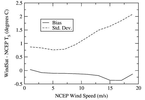
Fig. 7. Difference between the WindSat T_S retrievals and NCEP T_S results versus NCEP wind speed.
