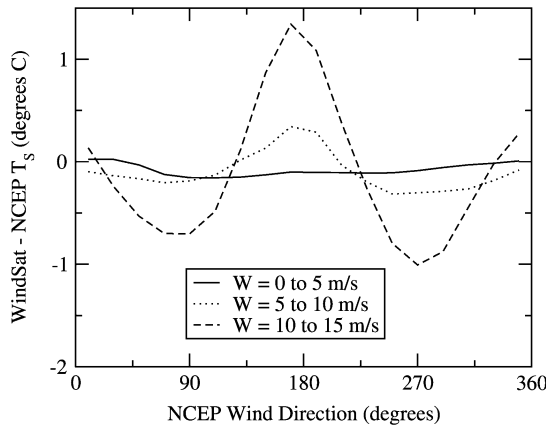
Fig. 9. Bias difference between the WindSat T_S retrievals and NCEP T_S versus NCEP wind direction relative to the WindSat look direction for three wind speed ranges.
