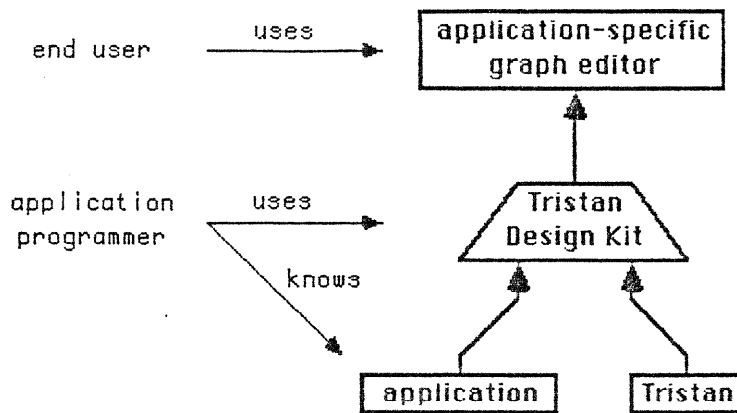
Figure 5-8: Usage of TRIKIT
