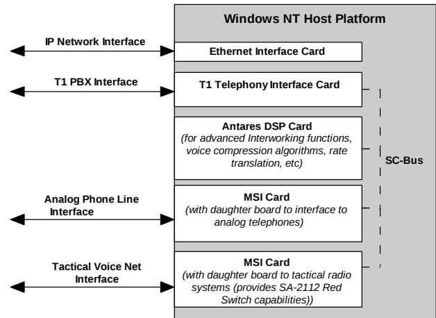
Fig. 2. – Phase II ELB Voice Gateway Platform
