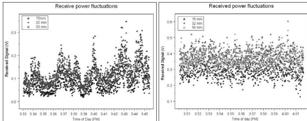
Fig. 7 a,b: Samples of voltages measured off of the 15mm, 32mm, and 50mm apertures. Fig. 7a(left) shows significant voltage fluctuations due to beam wander in the transmitter beam at best collimation, with the beam intentionally aimed off-center. Fig. 7b(right) is a sample the beam was centered on the receivers, and the impact of beam wander is minimized during the acquisition.
