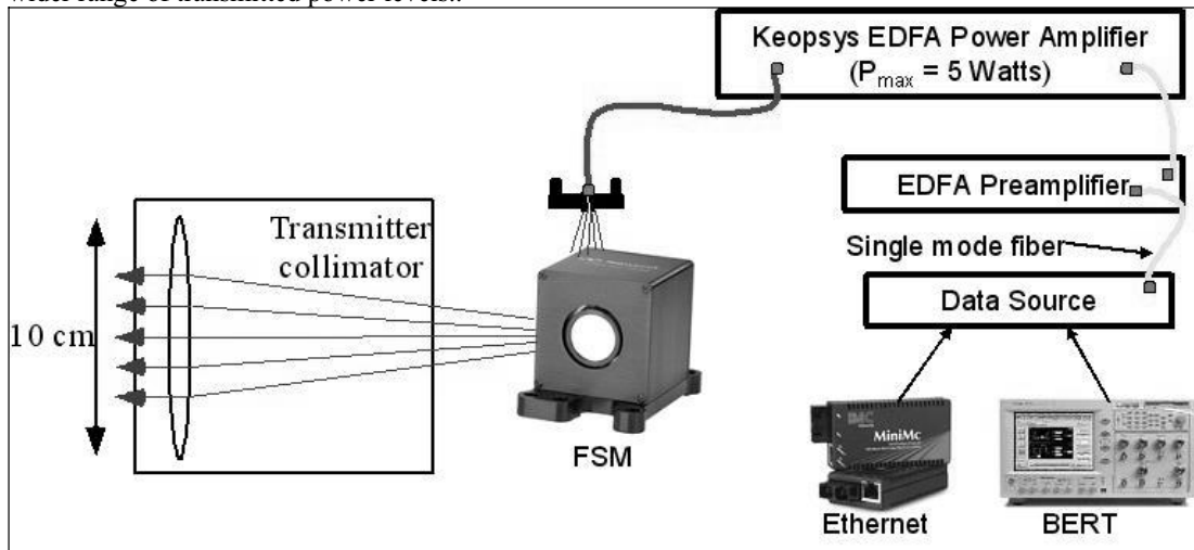
Fig. 2: Transmitter setup for lasercomm testing along the one-way link. In the Ethernet configuration, IMC Networks MiniMc transmitter is used as the data source. In the bit error rate testing setup, the Agilent 86130 or Anritsu ME522A BERT is used to generate a pseudorandom data stream.
