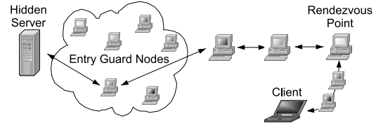
Figure 5. Use of Entry Guard Nodes
