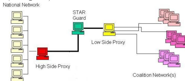
Figure 4 - Proposed Coalition Architecture with Guard
