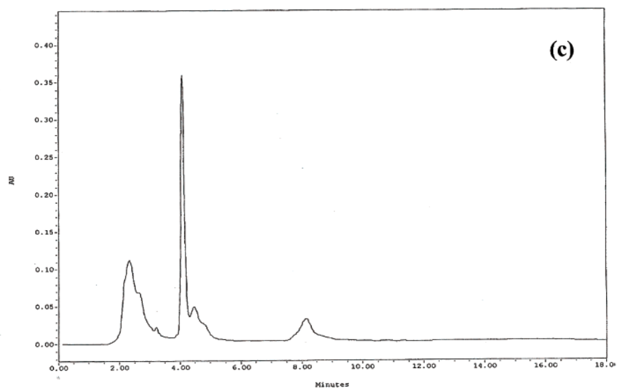
FIGURE 3. Parts (a) and (b) show the chromatogram and 14 C fraction distribution, respectively, under anaerobic conditions prior to thiol addition. Parts (c) and (d) show the chromatogram and 14 C fraction distribution, respectively, under anaerobic conditions after thiol addition
