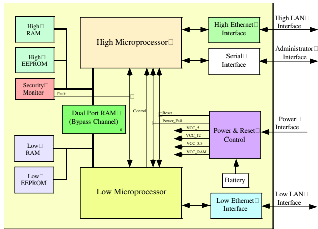
Figure 4: Network Pump™ hardware architecture
