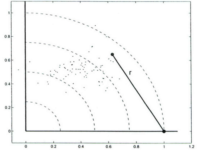
Figure 20. Example of a normalized Taylor diagram. Using polar coordinates, the ratio of the standard deviations of model and observed temperature tendency (radial coordinate) and the correlation angle \theta are plotted for each location and each year. The normalized error is the distance r from each point to the location of a perfect correlation (on the x-axis) and a ratio of one. See text for explanation.
