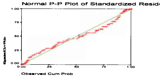
Figure 7. (U) The normal probability plot of the residuals.
