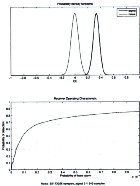
Figure 6. Statistics for a signal buried in noise (SNR = 0.32) for CC.
