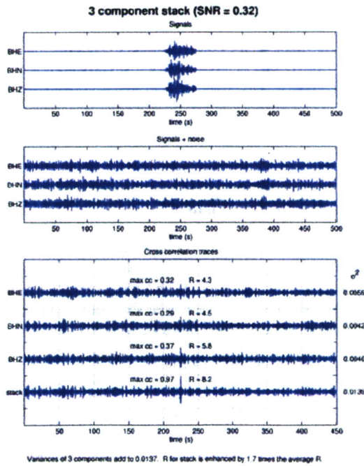
Figure 5. Three components enhance the detection spike.
