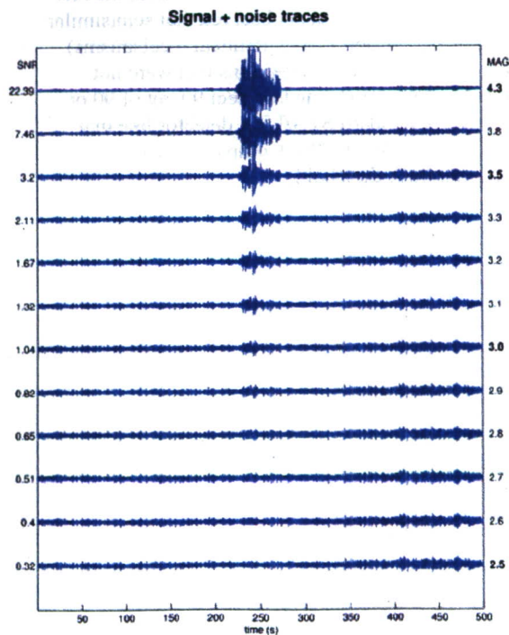
Figure 1. Lg-wave signals embedded in increasing noise.
