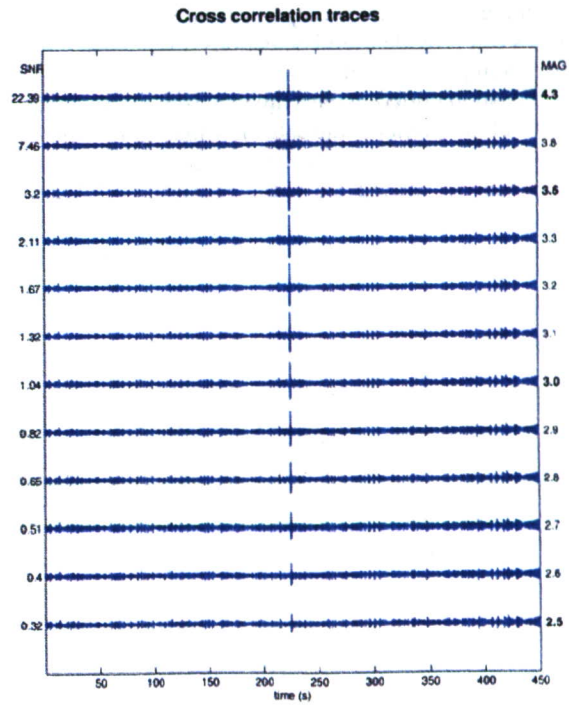
Figure 2. Cross correlation traces corresponding to Figure 1.
