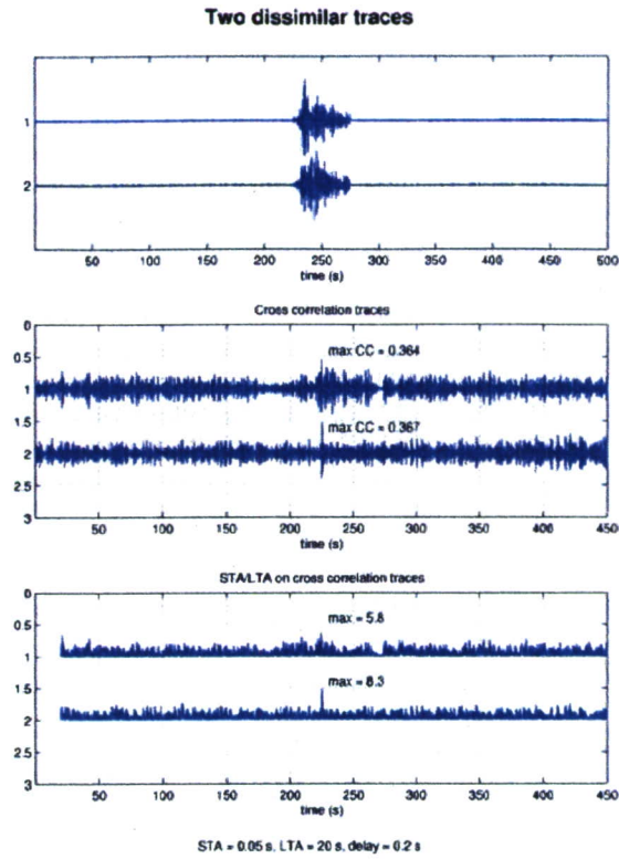
Figure 4. Two dissimilar traces would produce a false alarm with CC but not with a scaled CC.
