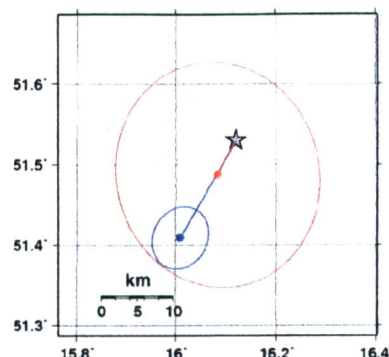
Figure 7. Relocation and 90% uncertainties of a Lubin GT1 event (star) using independence assumption (blue) and accounting for correlated errors (red).
