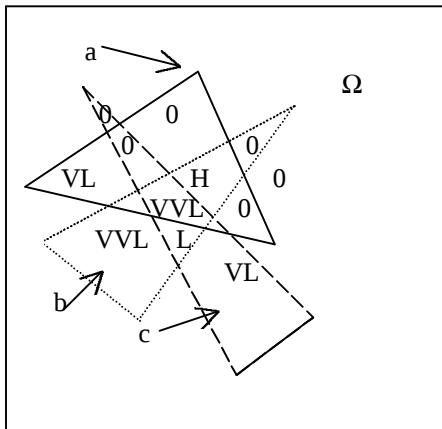
Figure 1. Example for conditional probability extension of classical transitivity-syllogism problem where premise set has high conditional probability values, but conclusion has a low (or even zero) conditional
