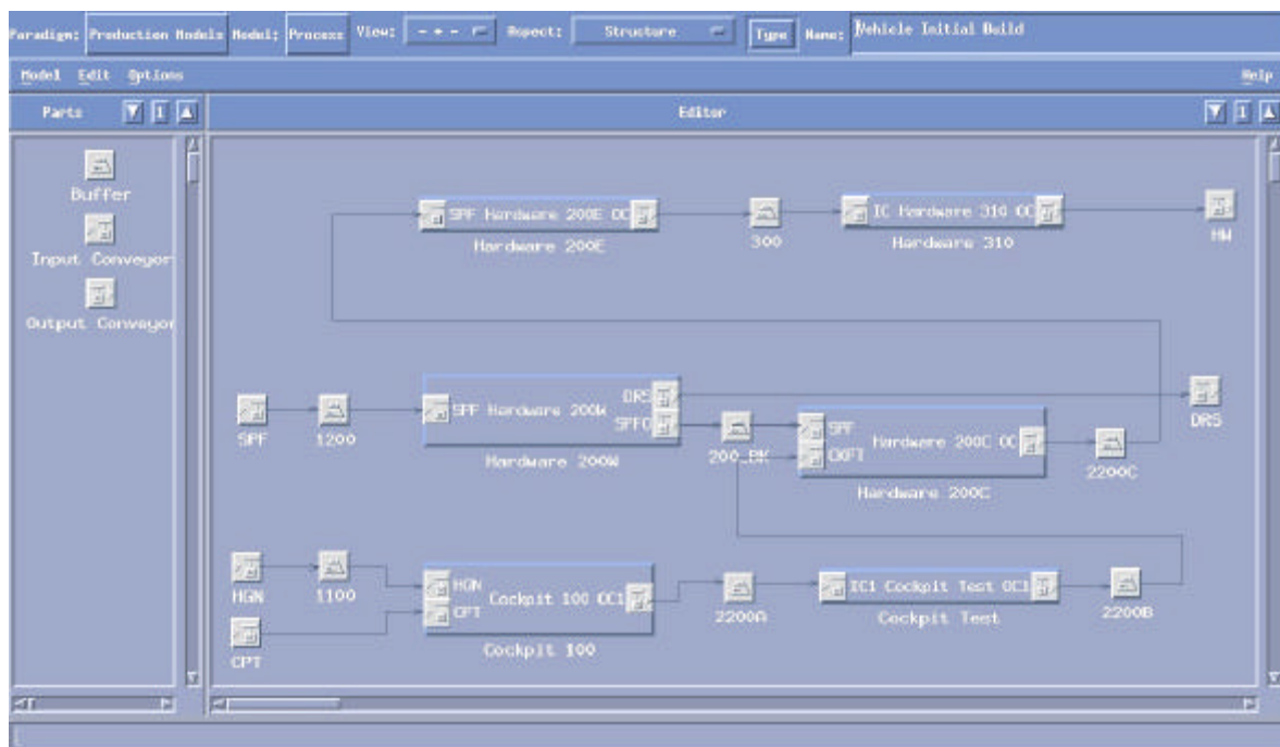
Figure 4: SSPF Model
